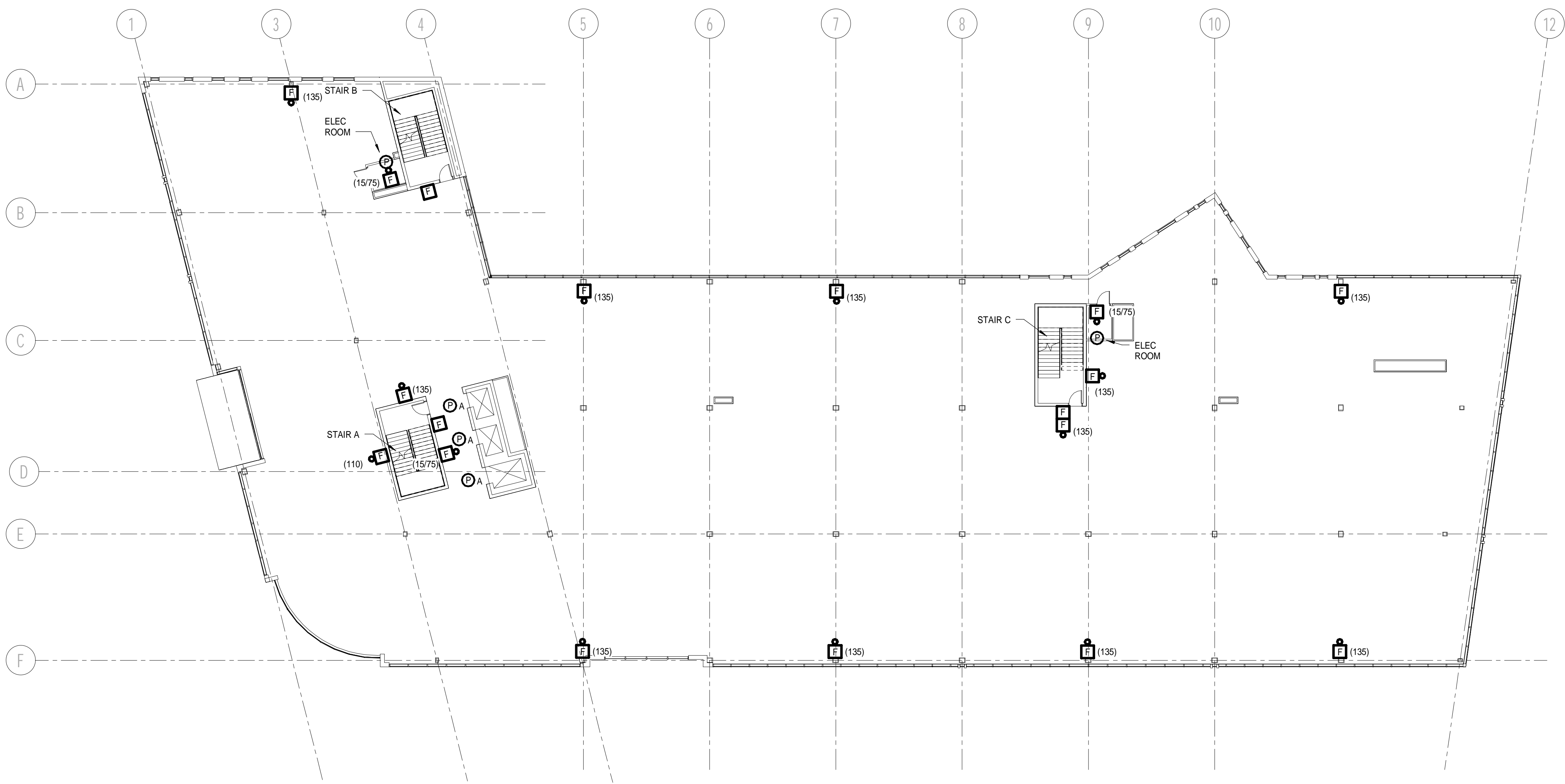
2ND FLOOR SYSTEMS PLAN (A1) 1/16" = 1'-0"
