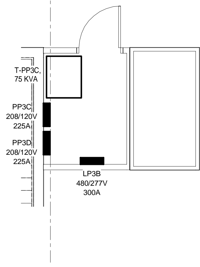
3RD FLOOR ELEC ROOM 2 POWER PLAN (H4) 1/4" = 1'-0"
