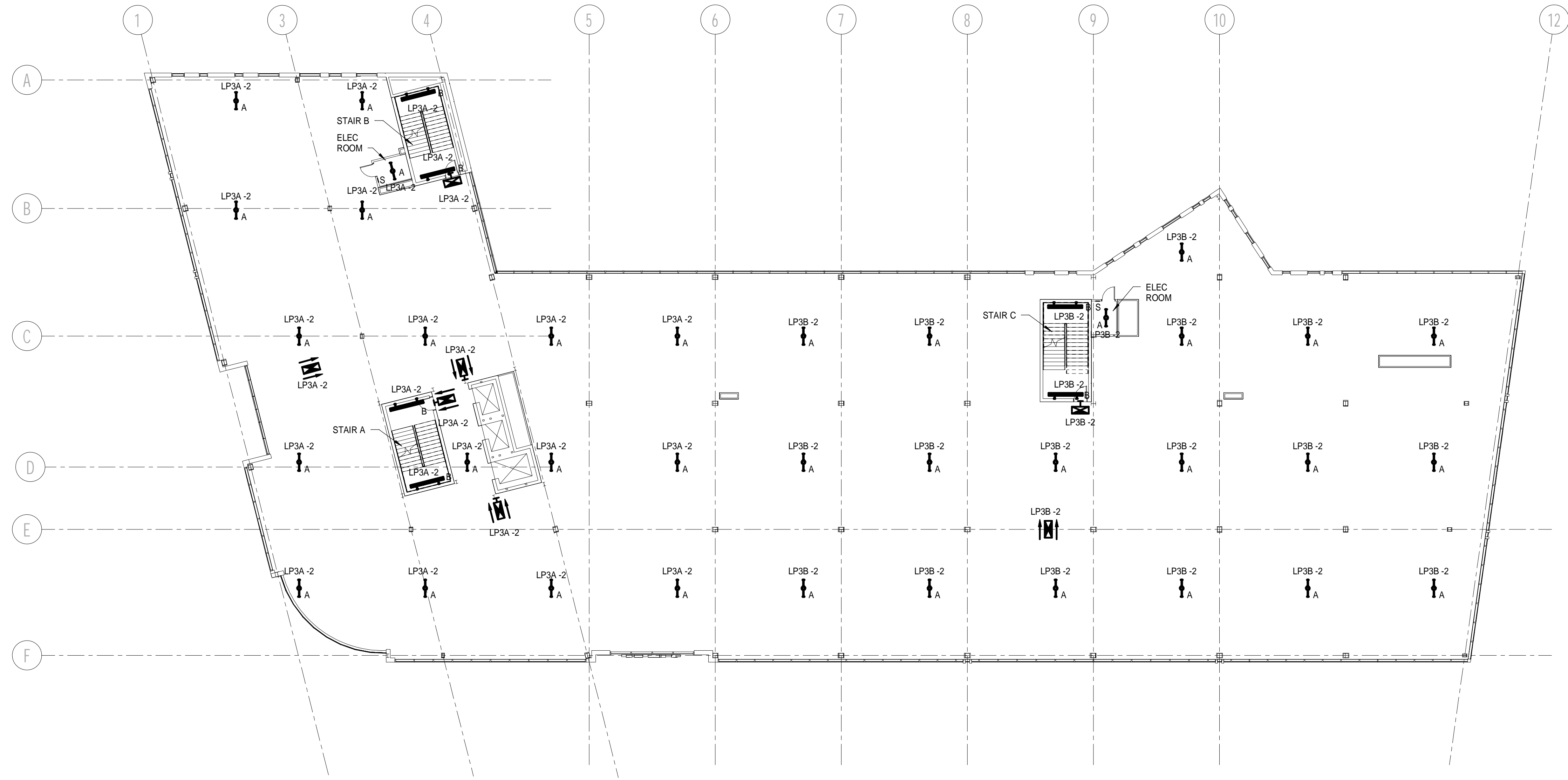
3RD FLOOR LIGHTING PLAN A1 1/16" = 1'-0"
