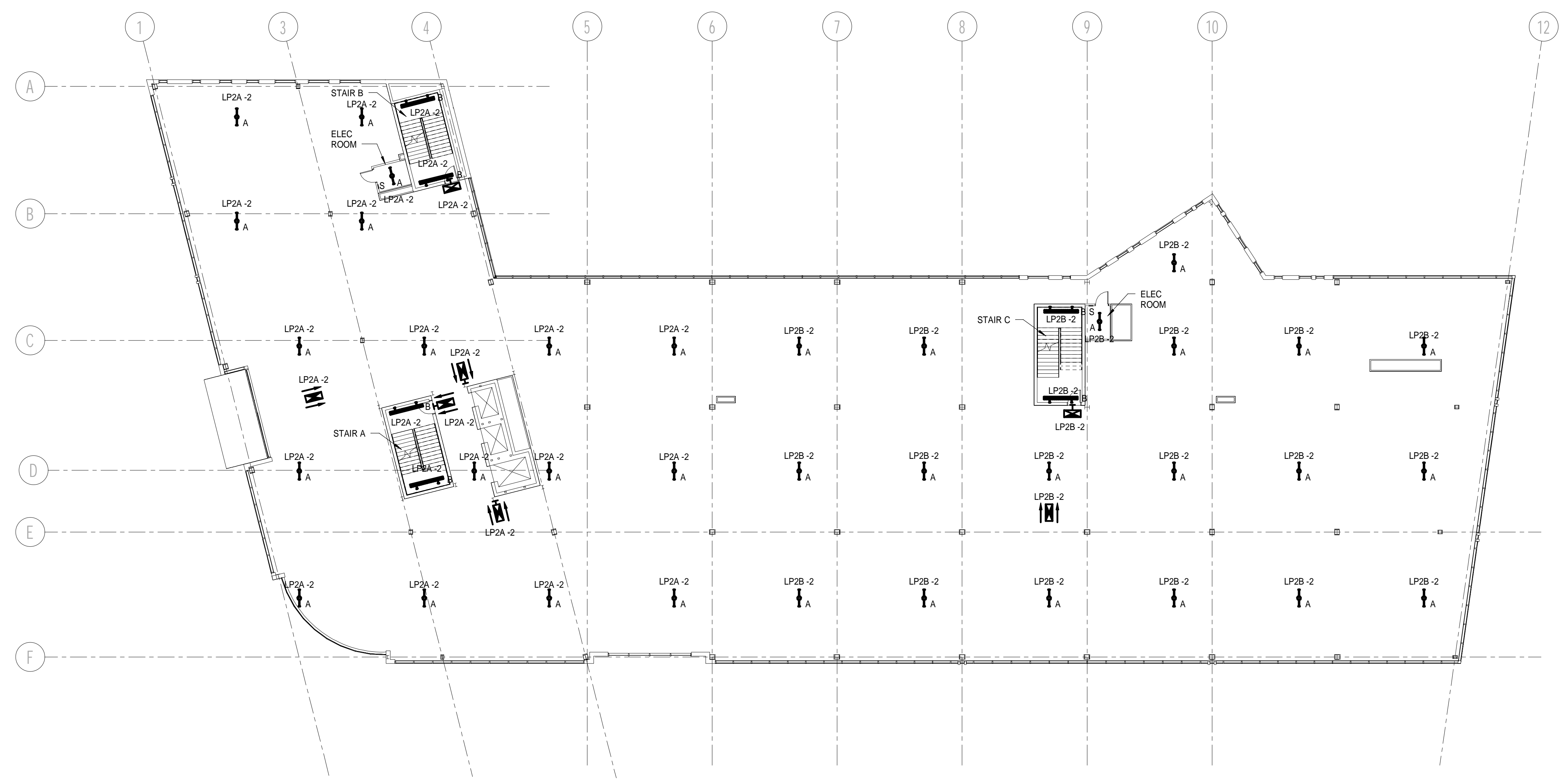
2ND FLOOR LIGHTING PLAN (A1) 1/16" = 1'-0"
