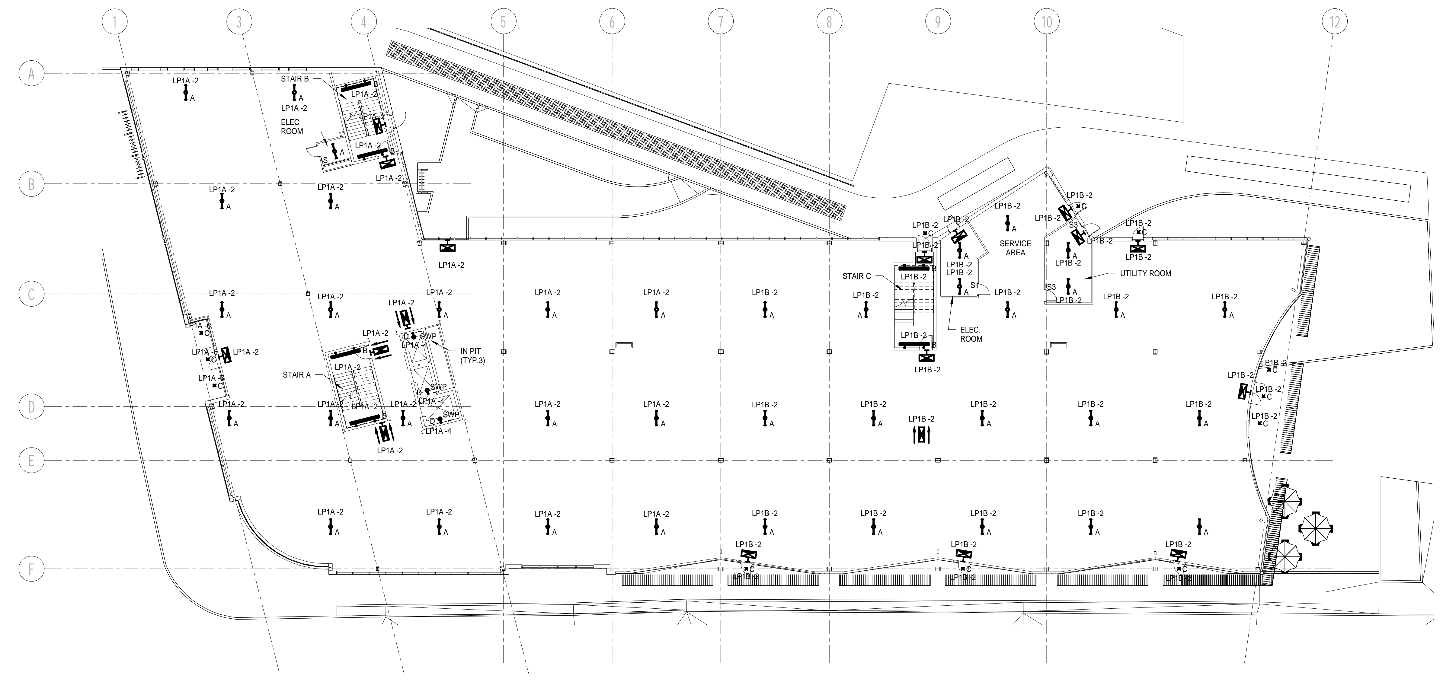
1ST FLOOR LIGHTING PLAN 1/16" = 1'-0" A1
