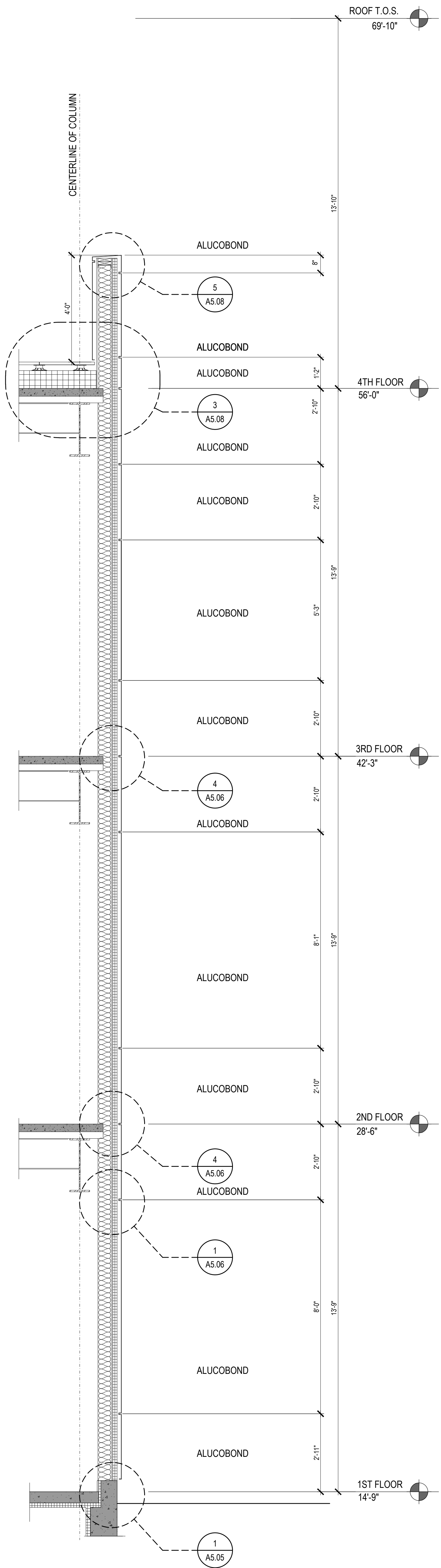
1 WALL SECTION
