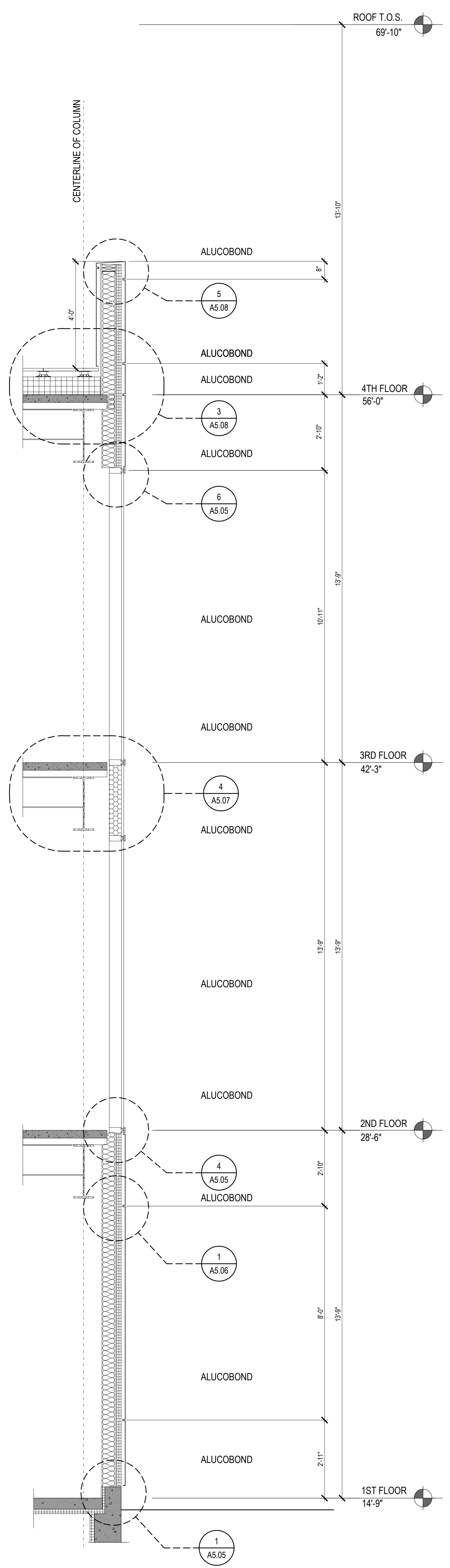
2 WALL SECTION
