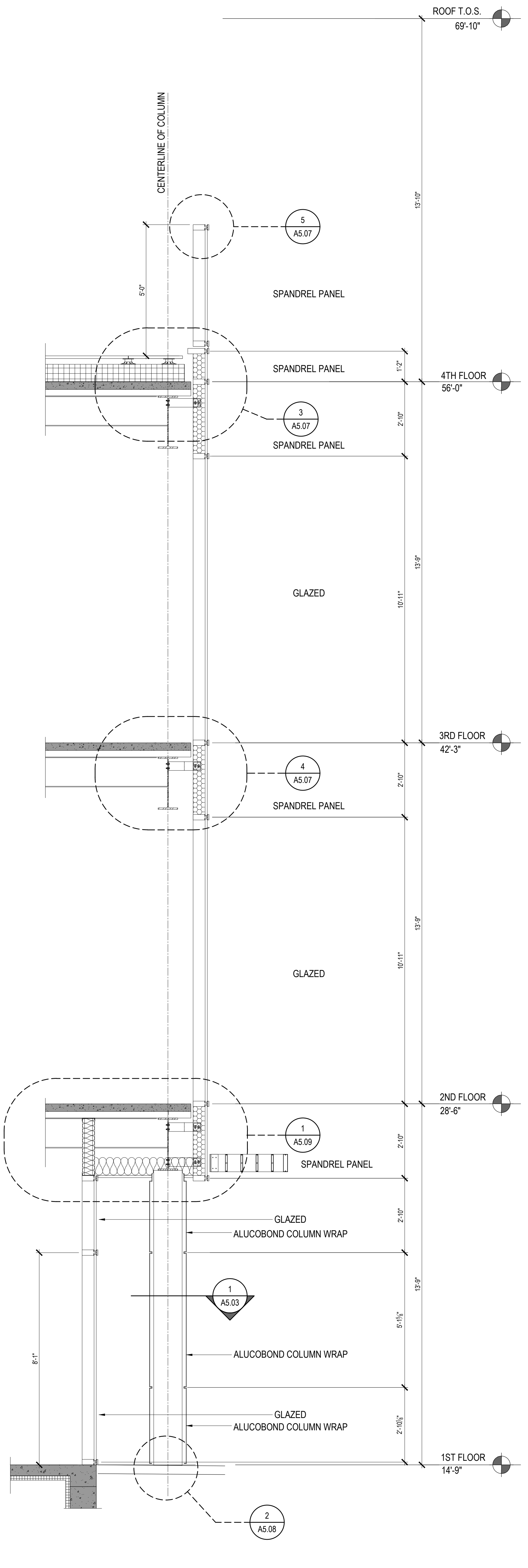
2 WALL SECTION
