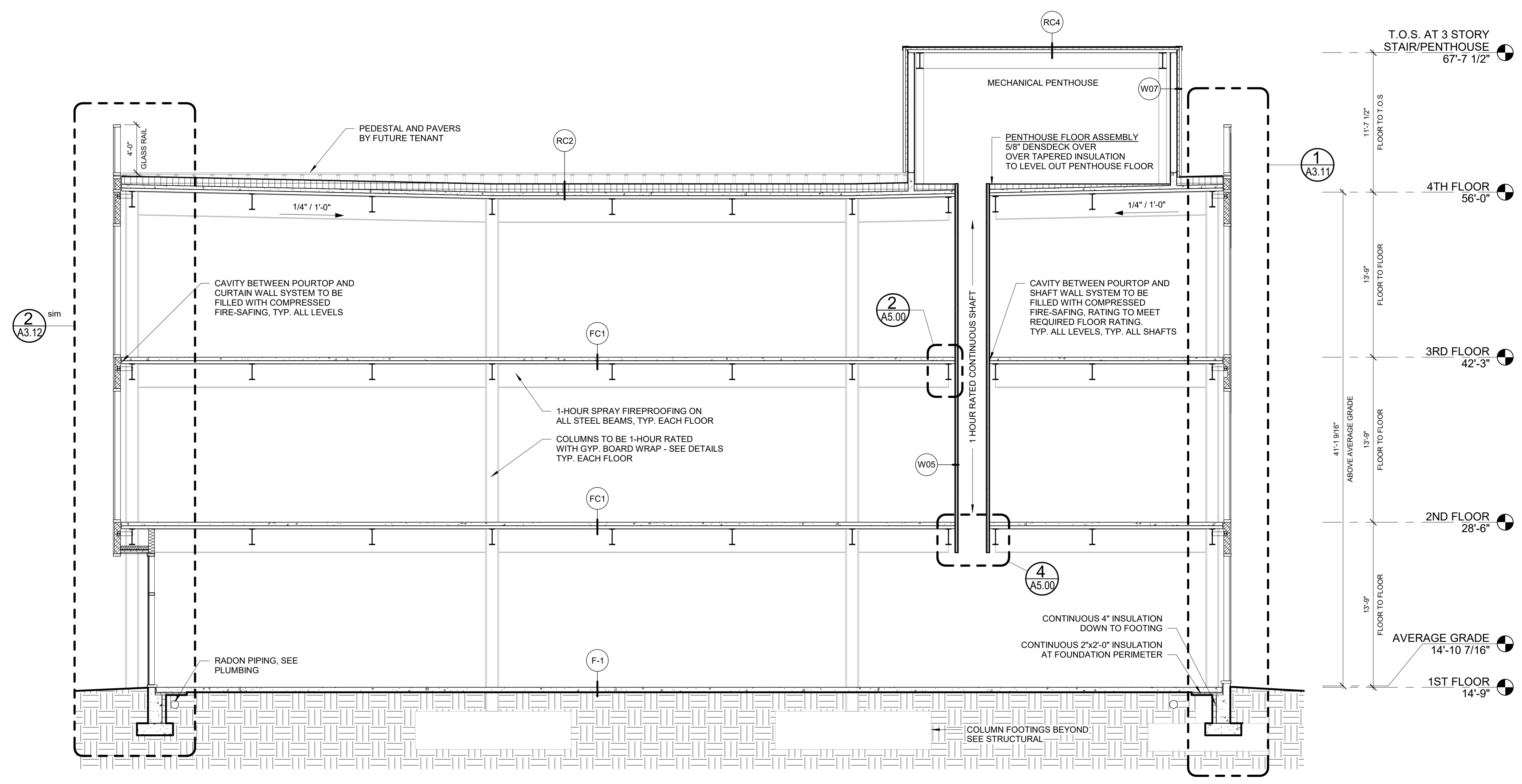
1 | SECTION AT THREE STORY BUILDING 3/16" = 1'-0"
