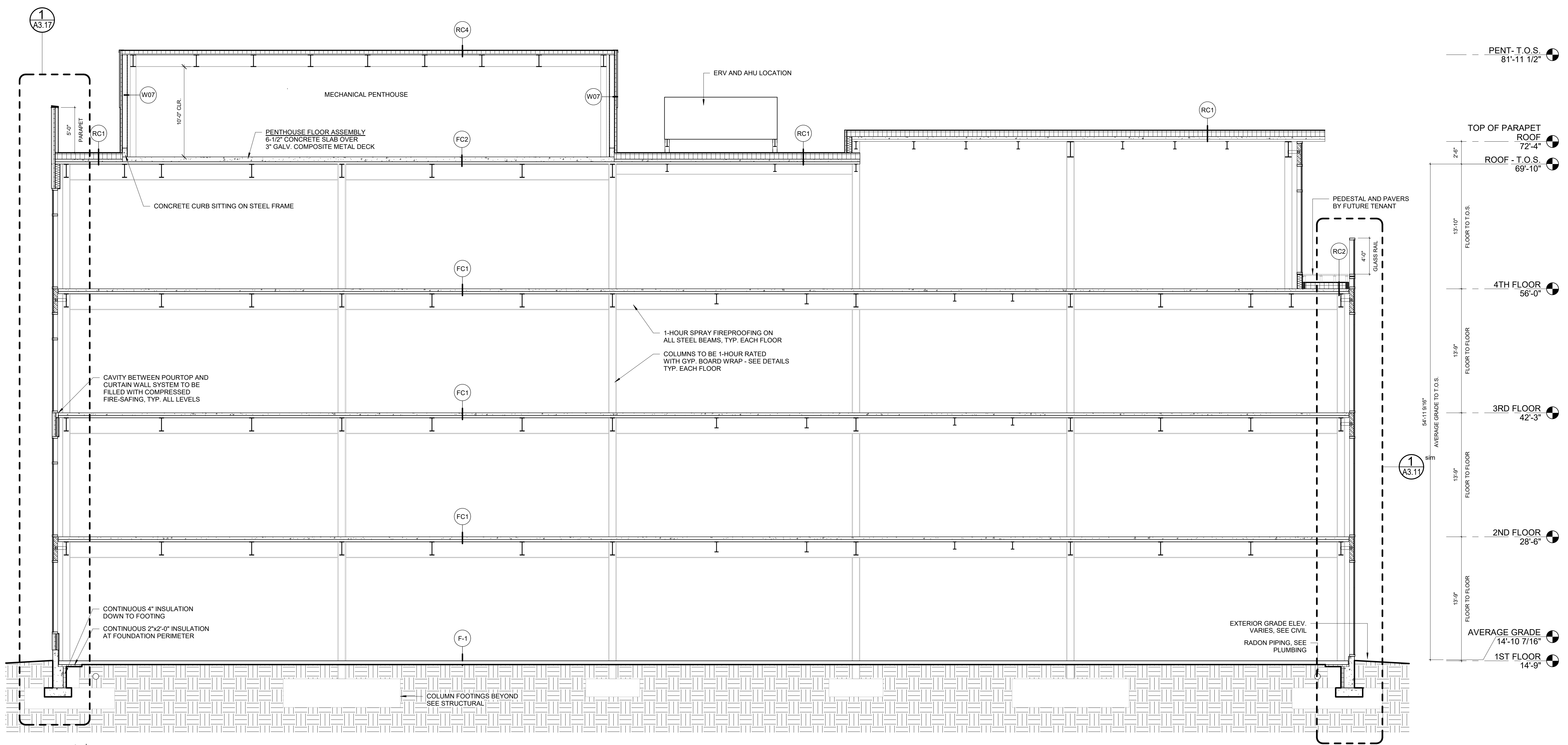
1 | CROSS SECTION AT FOUR STORY BUILDING 3/16" = 1'-0"
