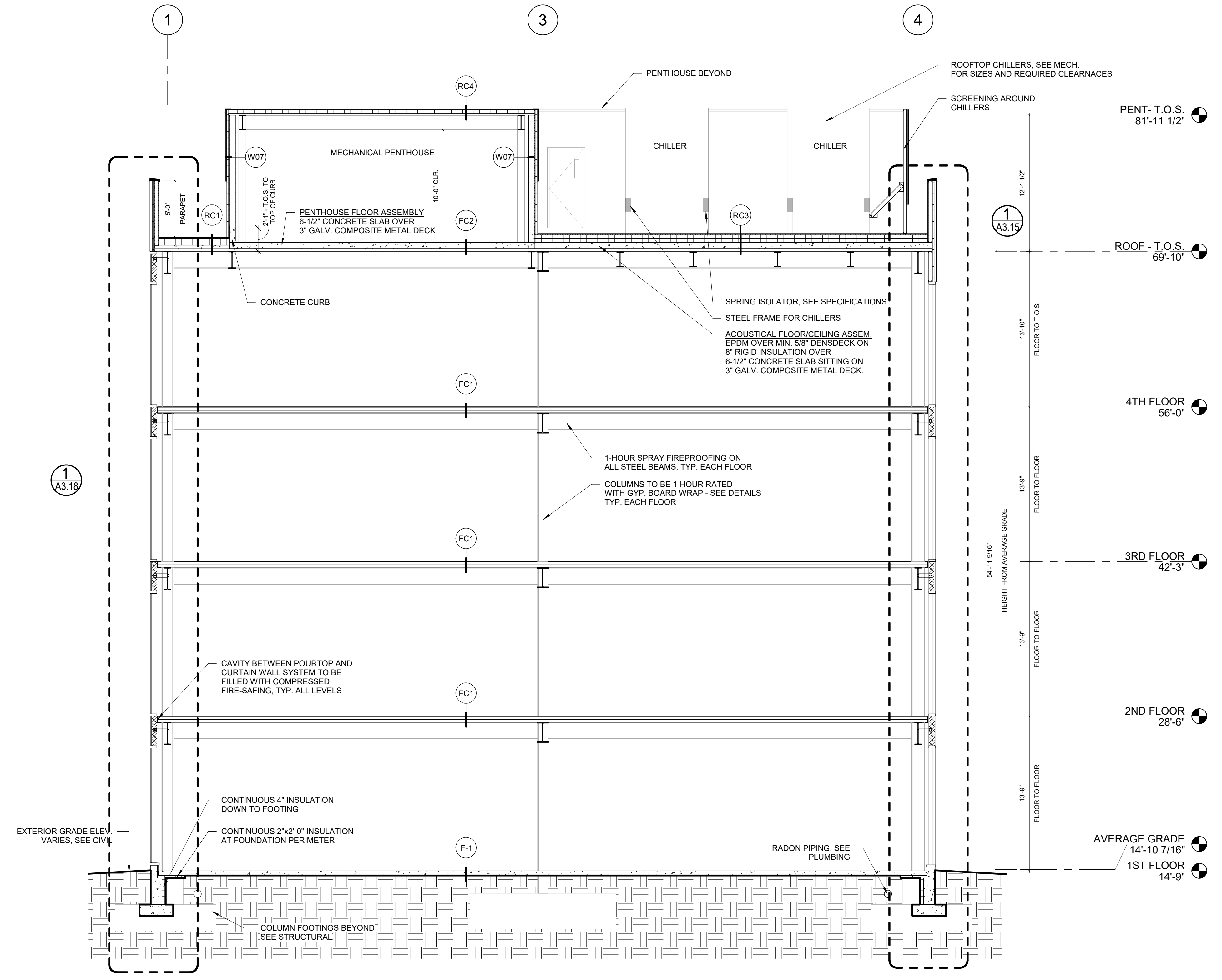
1 | SECTION AT FOUR STORY BUILDING 3/16" = 1'-0"
