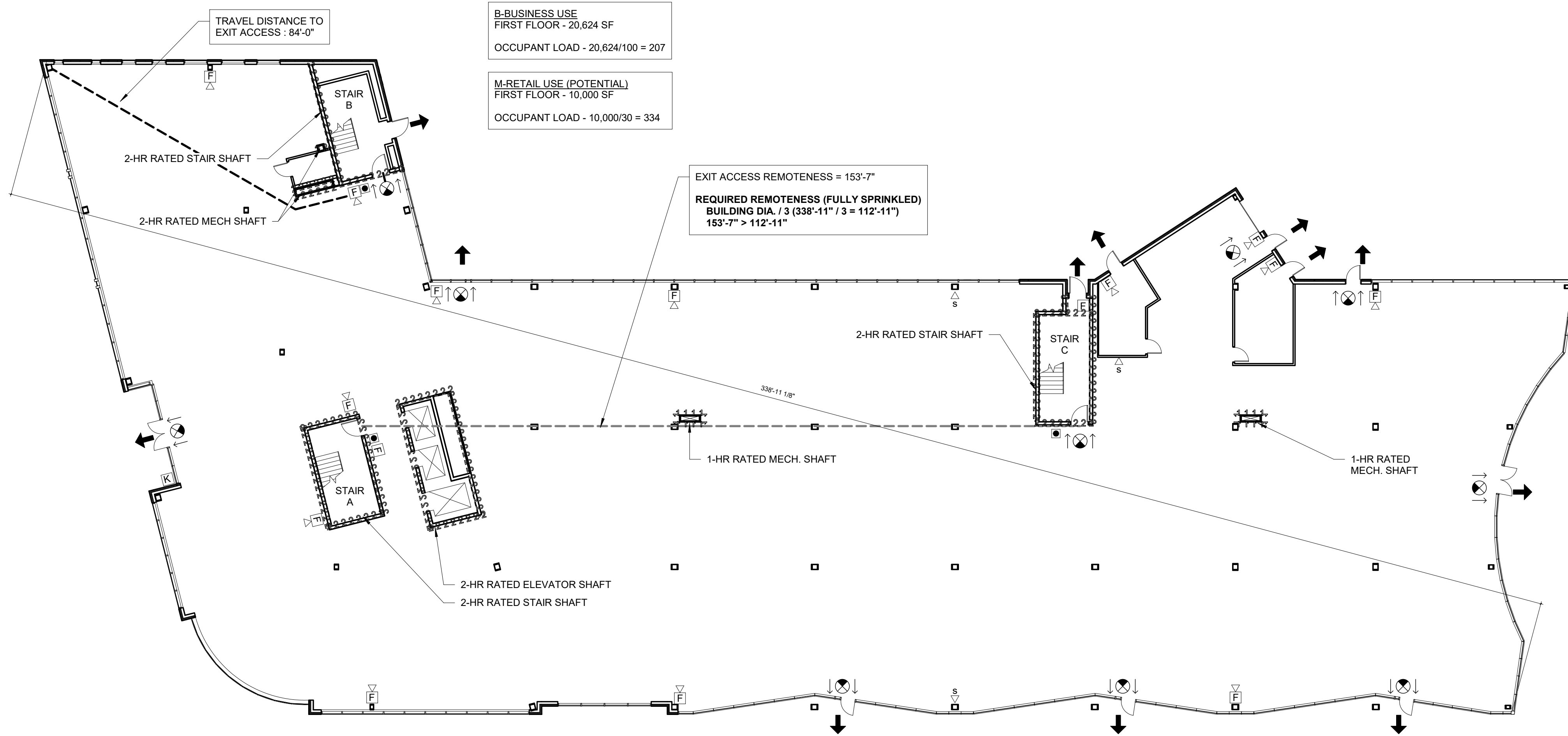
1 | 1ST FLOOR - LIFE SAFETY PLAN 1/16" = 1'-0"
