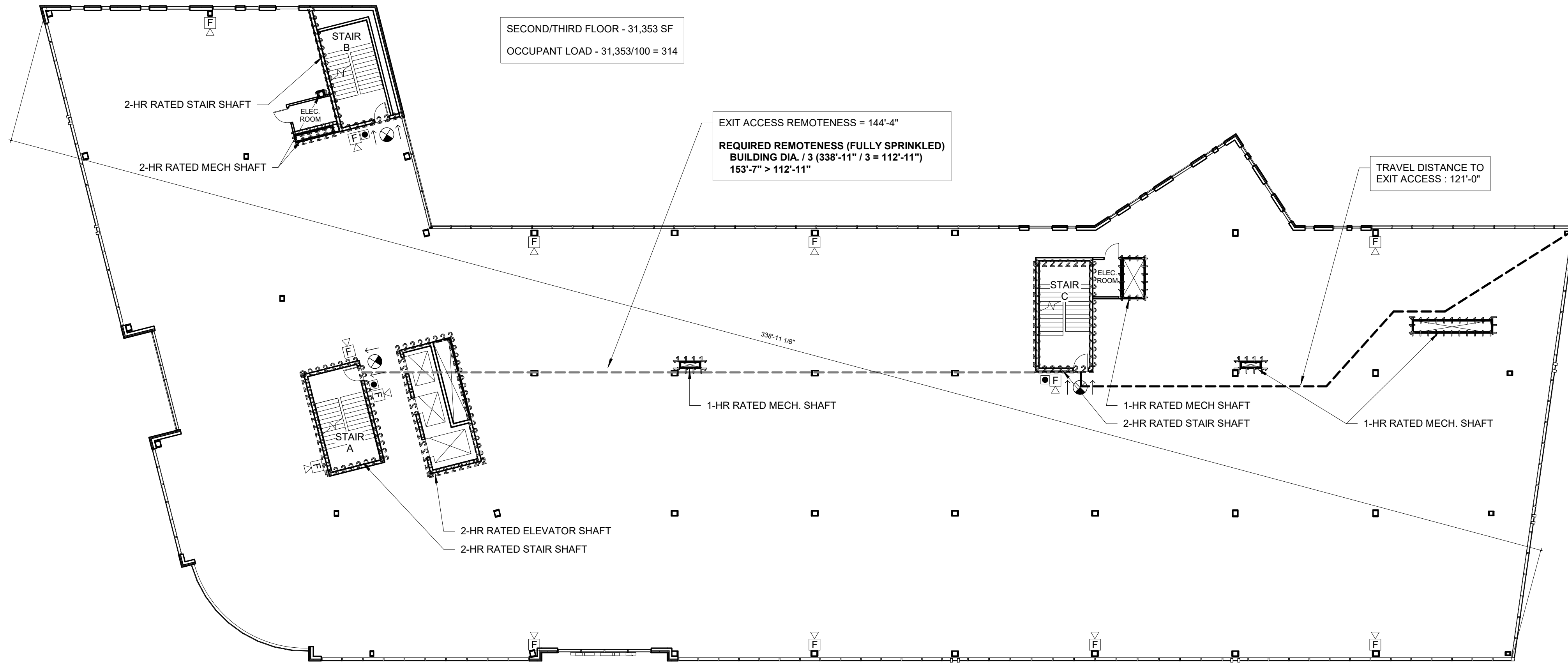
2 | 2ND AND 3RD FLOOR 1/16" = 1'-0"
