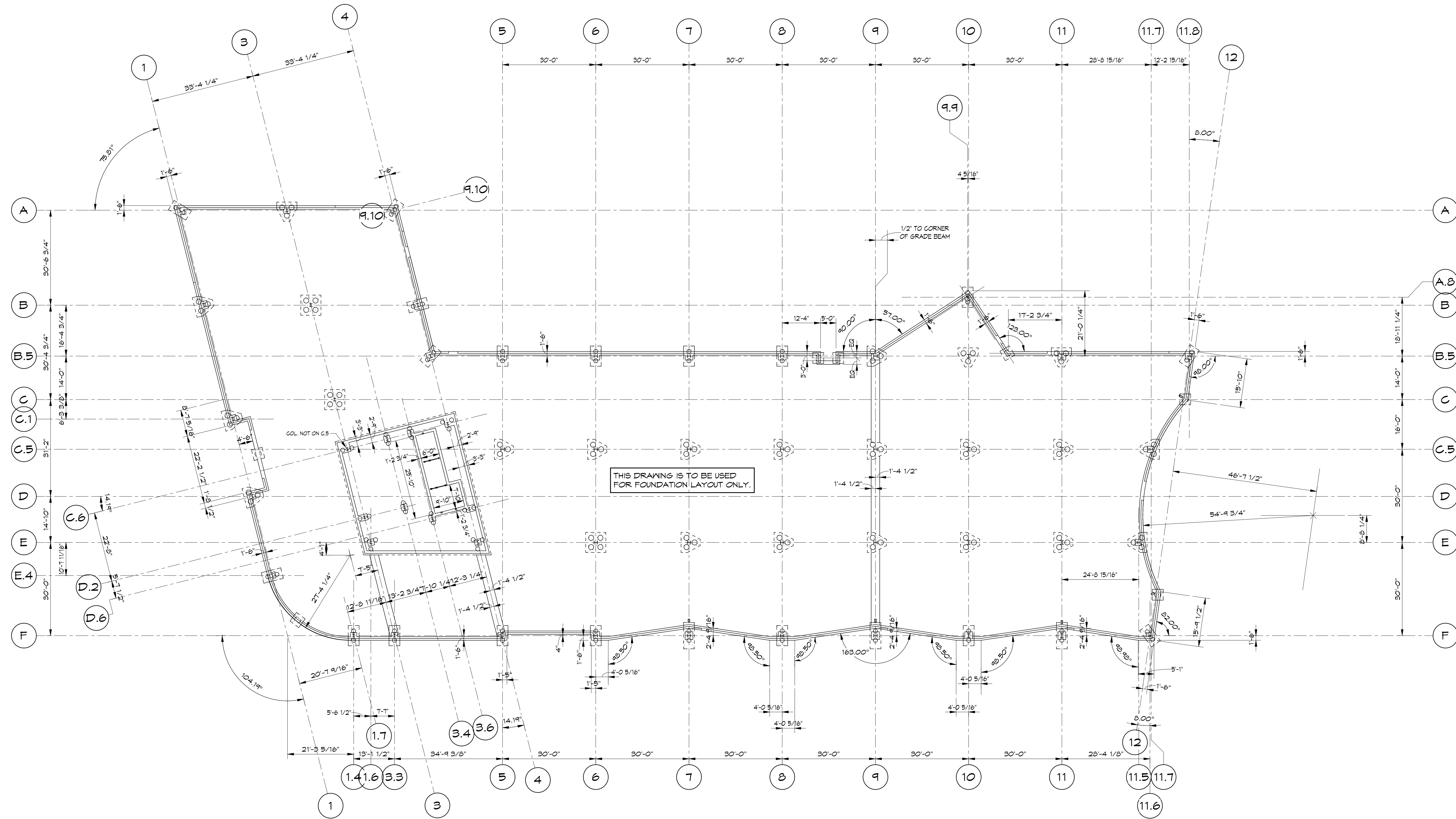
1 FOUNDATION LAYOUT PLAN 1/16" = 1'-0"
