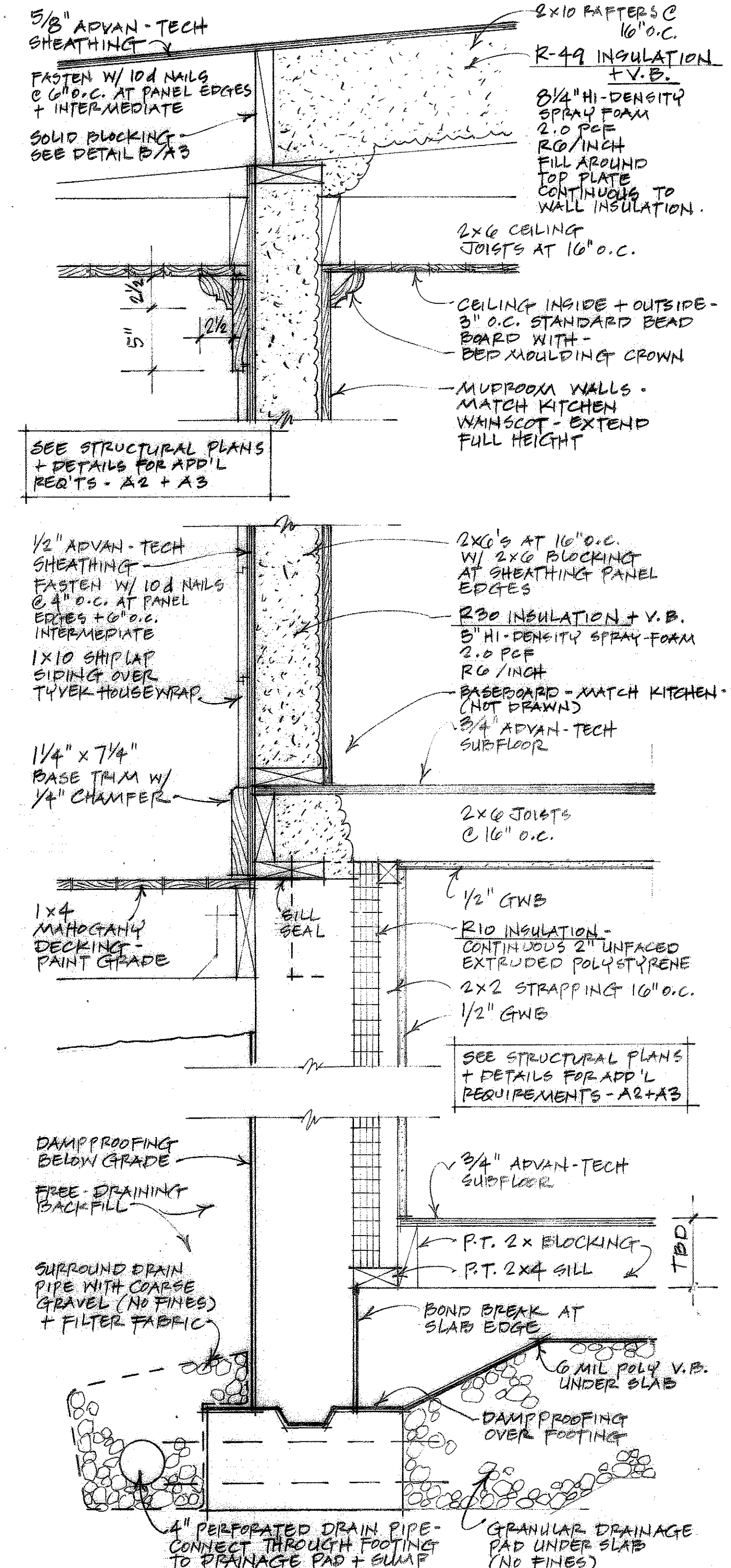
2 SECTION THROUGH MUDROOM. 1/2" = 1'-0"
