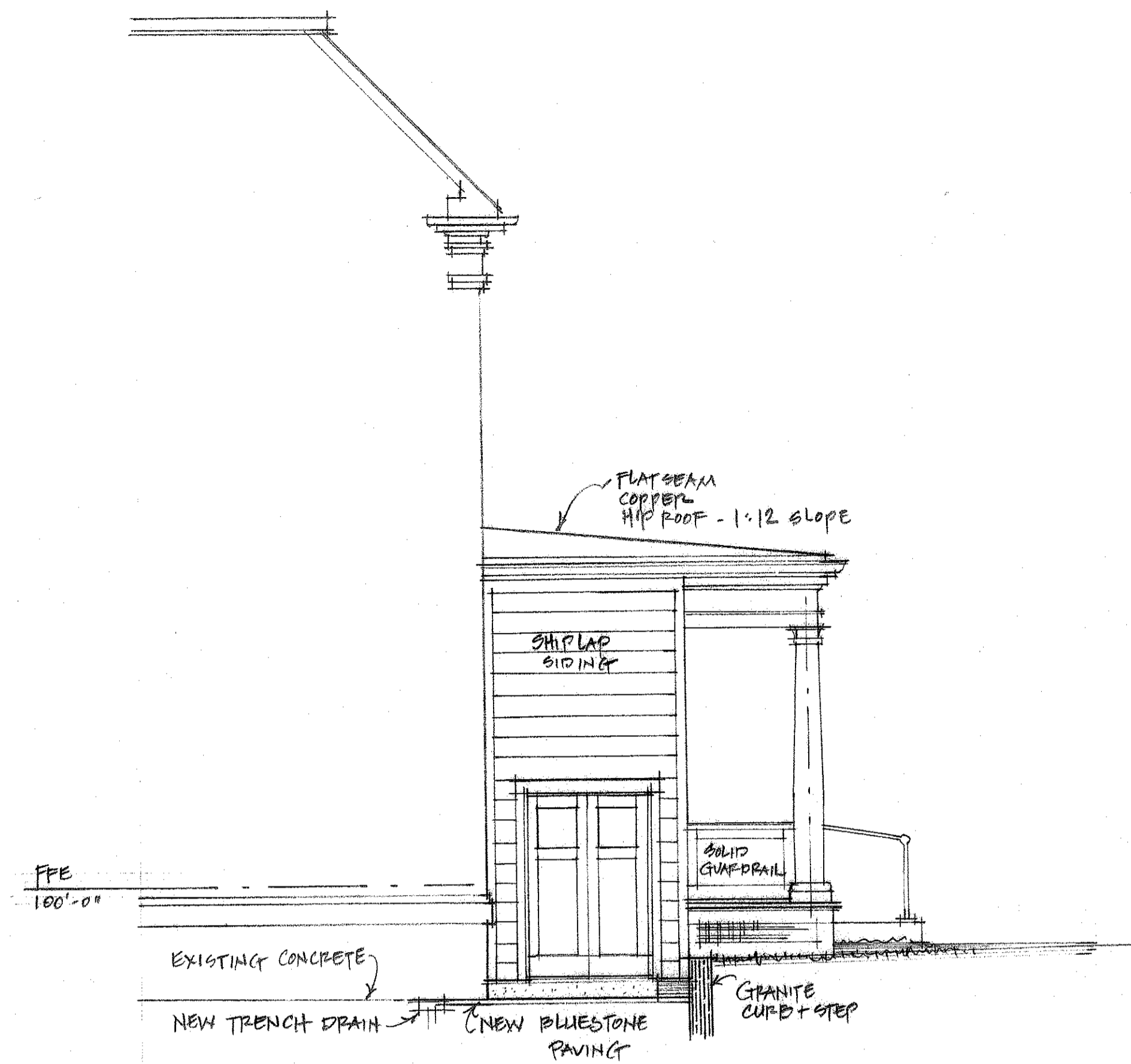
PROPOSED COURTYARD ELEVATION EAST - SITE SECTION B-B 1/4" = 1'-0"
