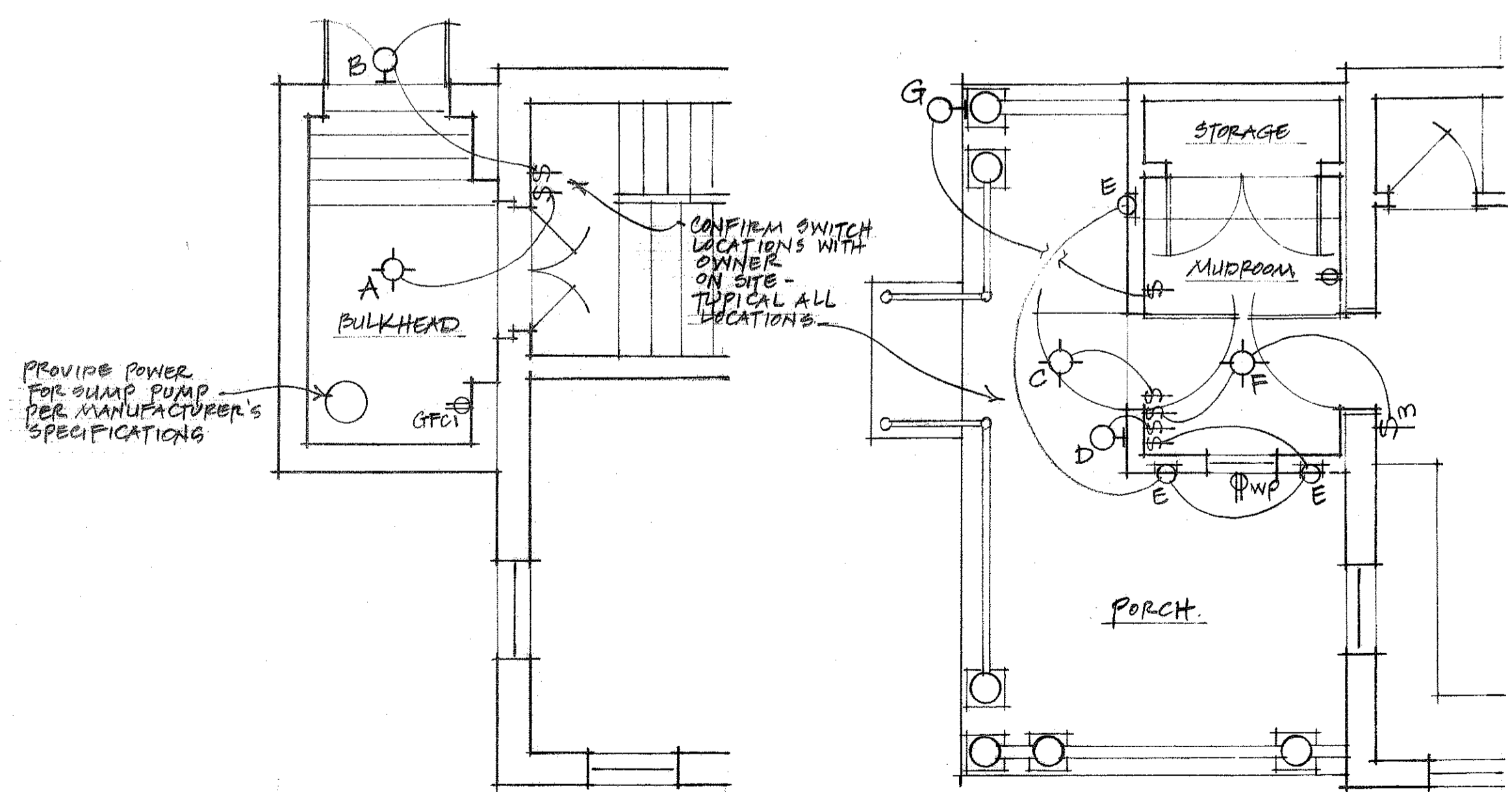
③ BASEMENT ELECTRICAL PLAN 1/4" = 1'-0"
