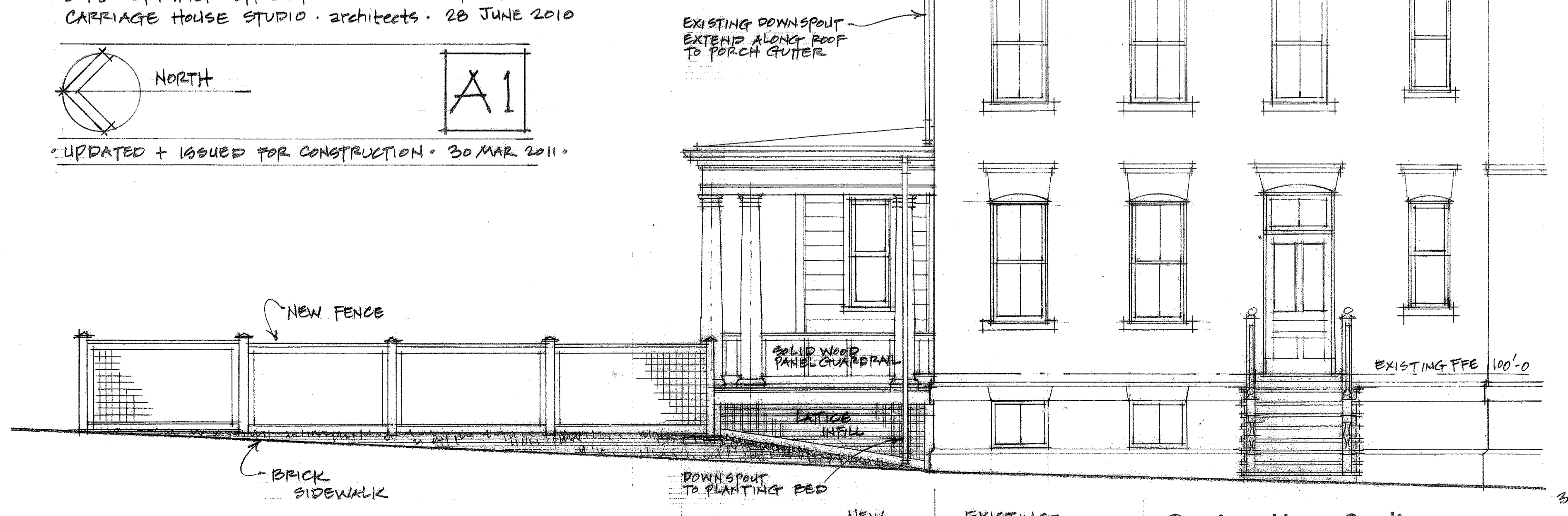
PROPOSED SIDE YARD ELEVATION WEST - VAUGHAN ST. ELEVATION
