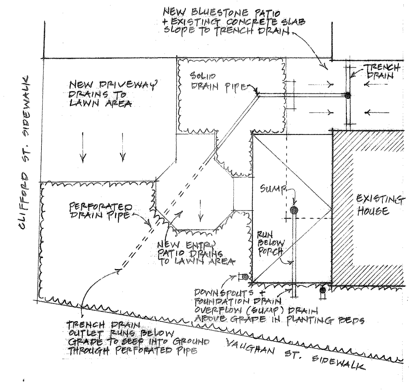
⑤ SITE DRAINAGE PLAN NO SCALE
