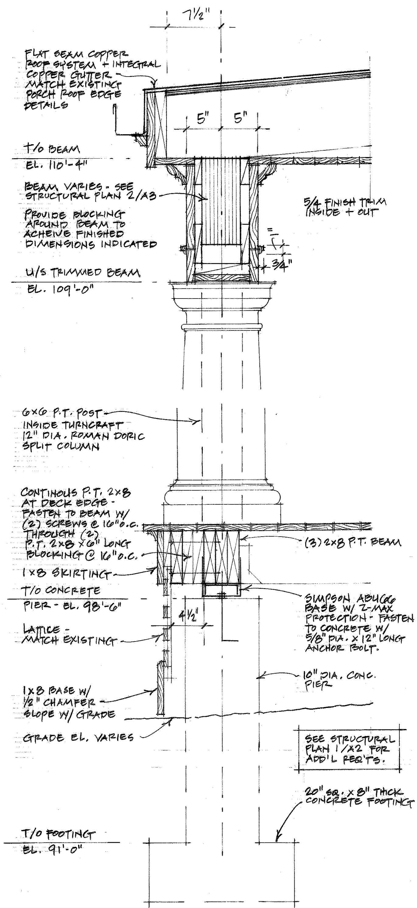
1 SECTION THROUGH PORCH. 1/2" = 1'-0"
