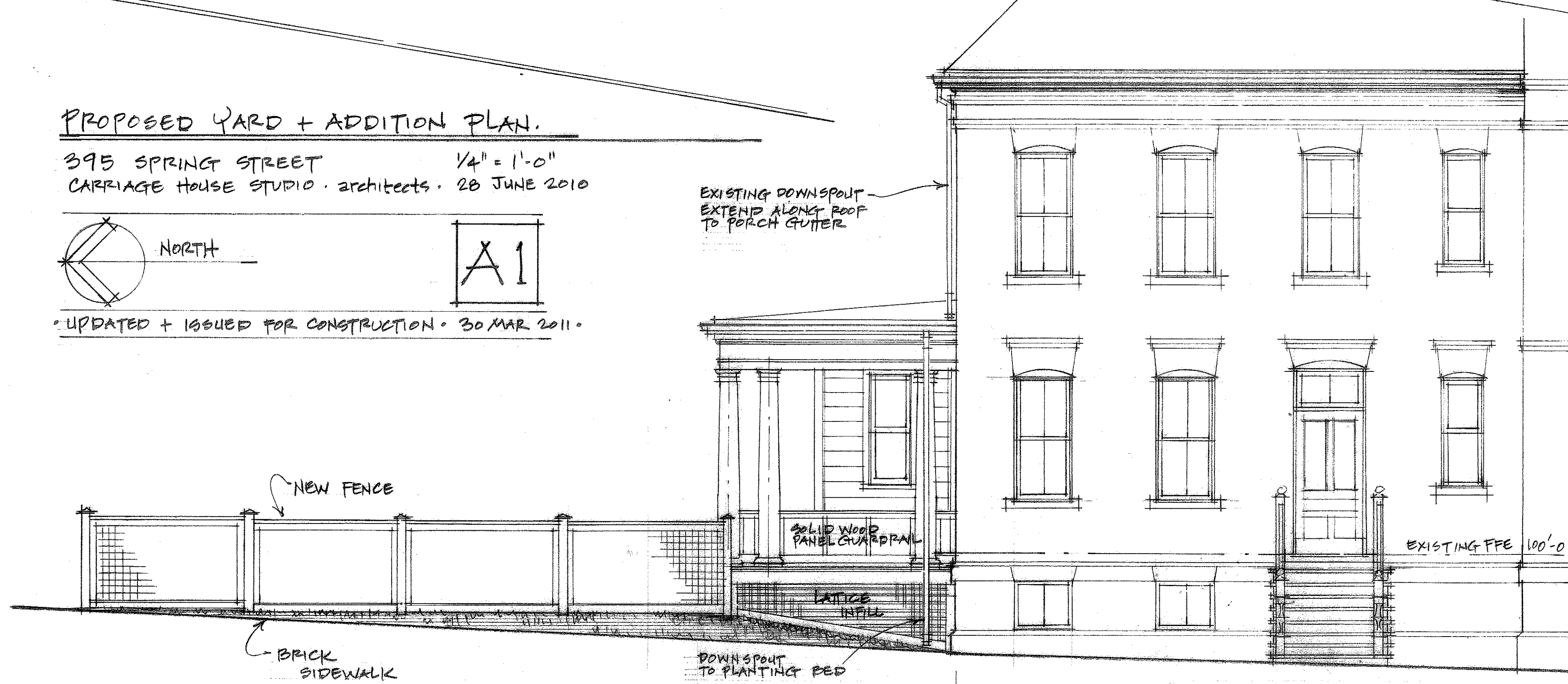
PROPOSED SIDE YARD ELEVATION
