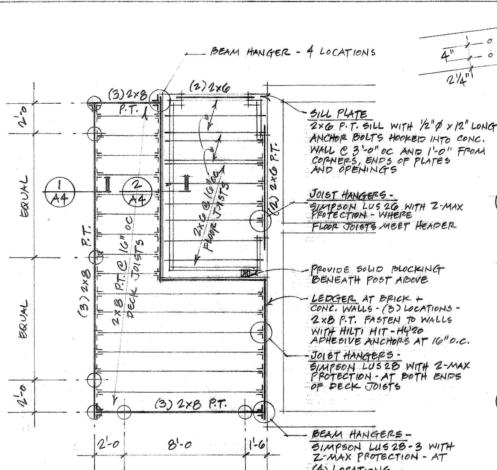
① FIRST FLOOR FRAMING PLAN. 1/4" = 1'-0"
