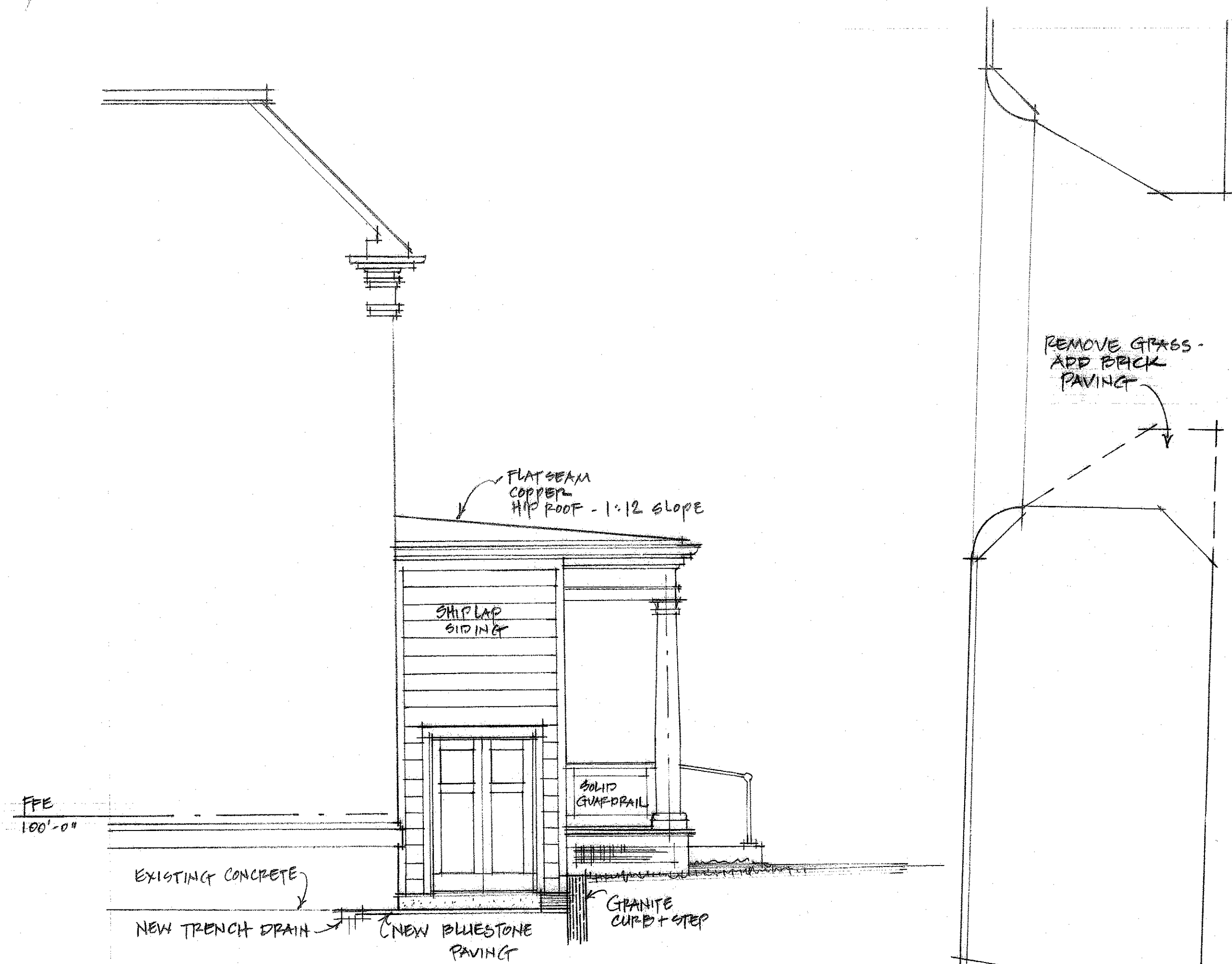
PROPOSED COURTYARD ELEVATION EAST - SITE SECTION B-B 1/4" = 1'-0"
