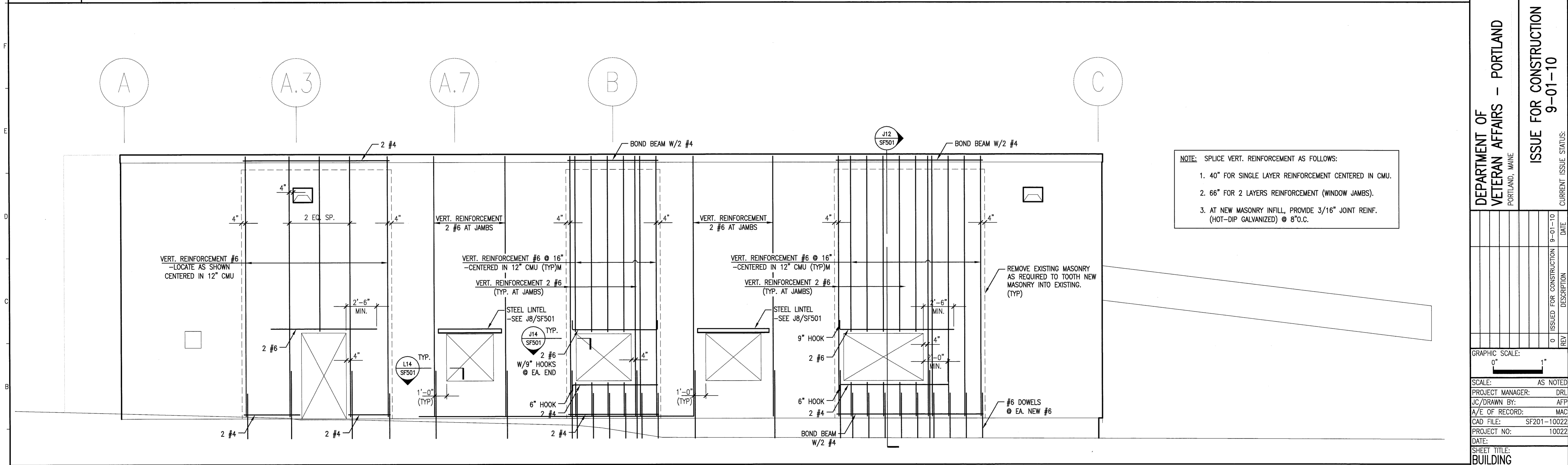
A1 WEST WALL REINFORCING ELEVATION
