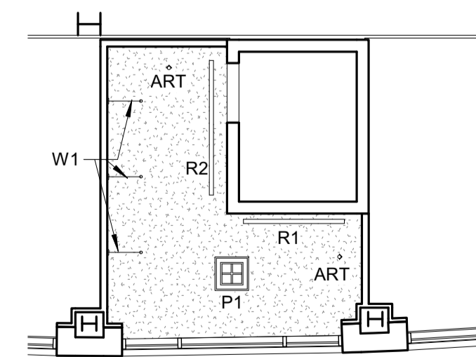
6 | LOBBY CEILING 1/8" = 1'-0"
