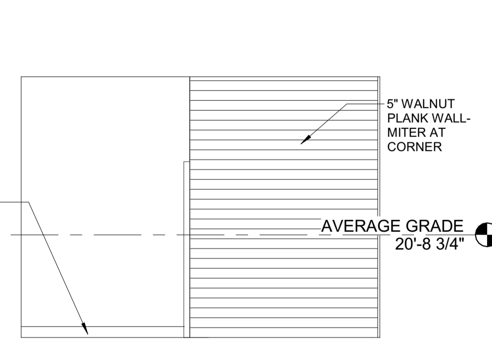
2 | LOBBY - INTERIOR ELEVATION 1/4" = 1'-0"
