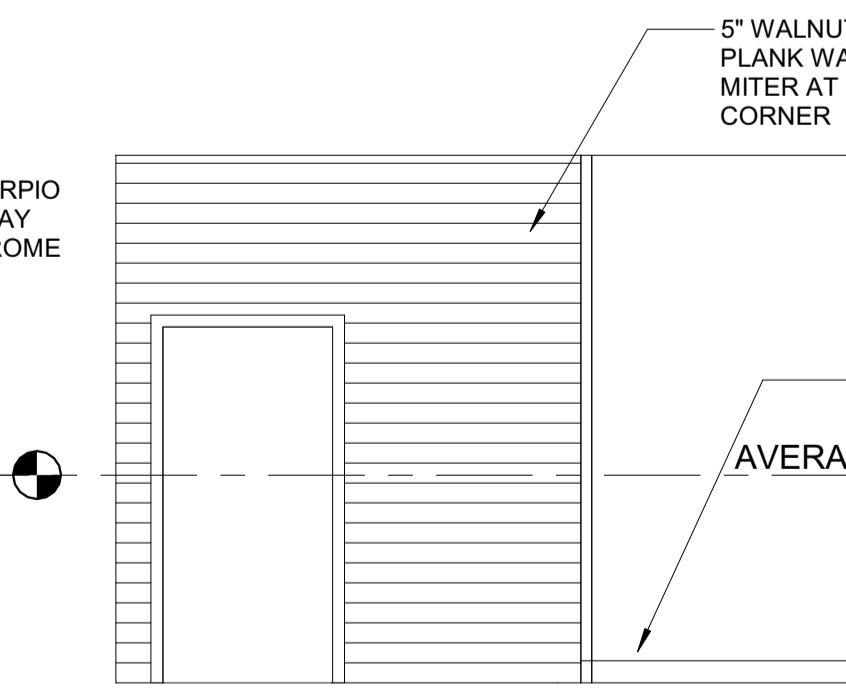
3 | LOBBY - INTERIOR ELEVATION 1/4" = 1'-0"
