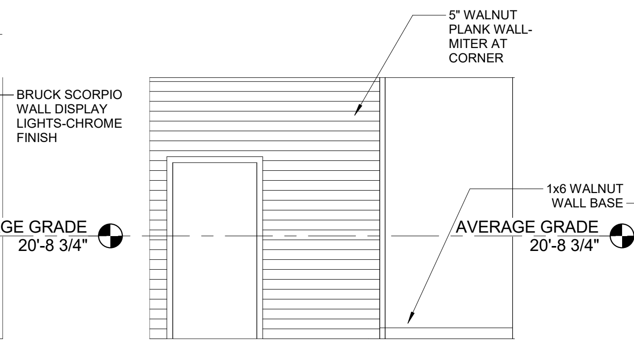
3 | LOBBY - INTERIOR ELEVATION 1/4" = 1'-0"
