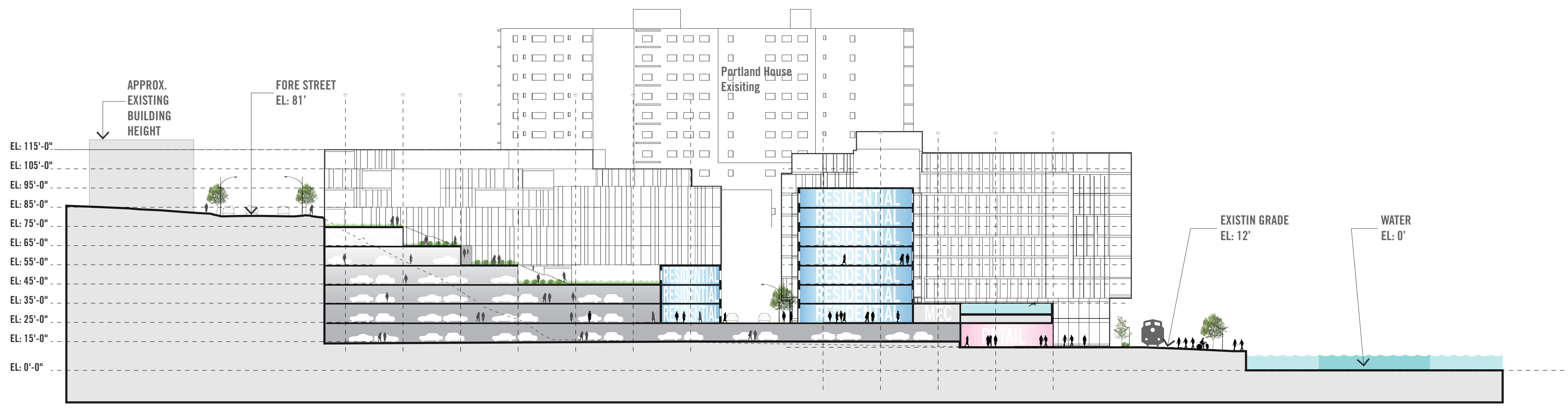
SCALE: 1"=40'-0" SECTION 11 FORE STREET DEVELOPMENT BLOCK 4 55' DEVELOPMENT BLOCK 5
