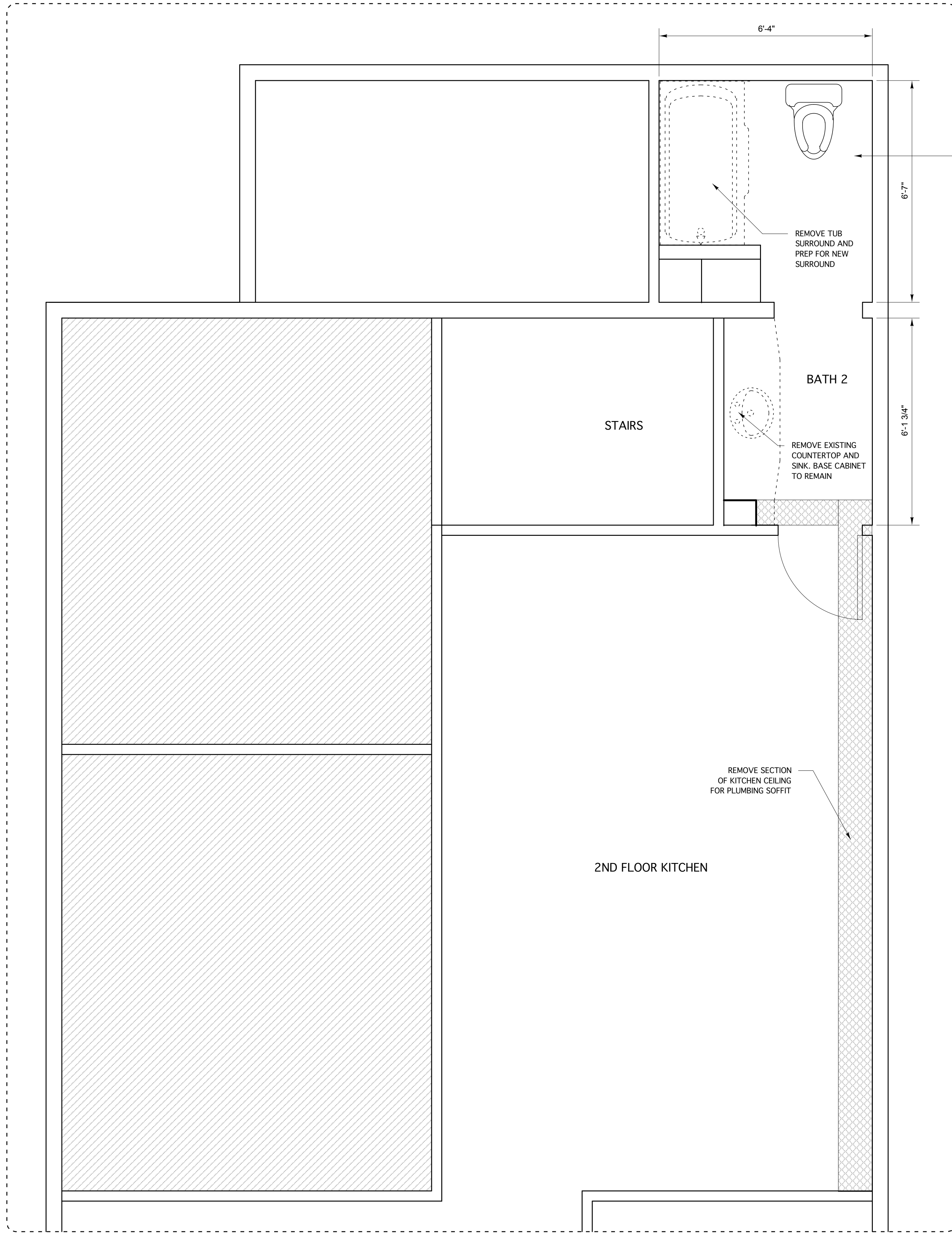
3 SECOND FLOOR DEMOLITION PLAN A2
