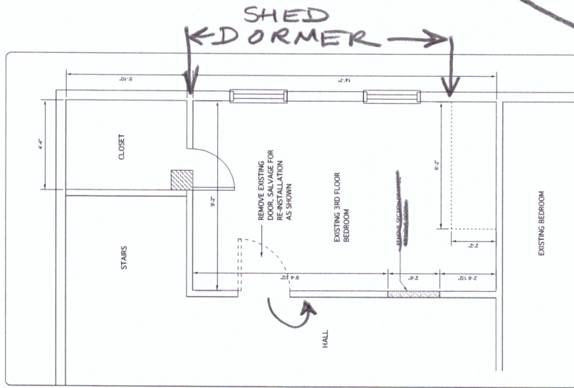
1 THIRD FLOOR DEMOLITION PLAN A3
