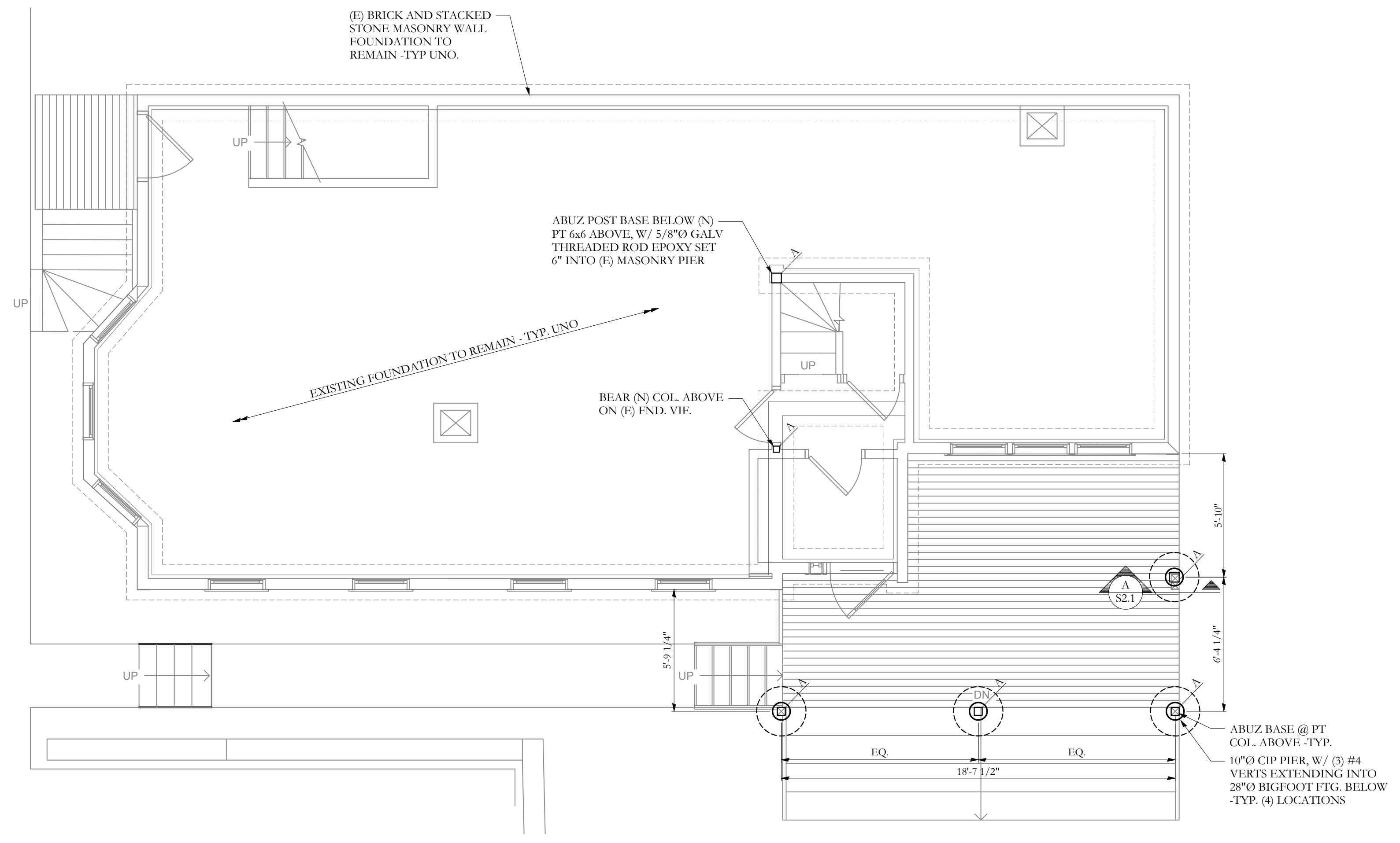
FOUNDATION PLAN SCALE 1/8"=1'-0"
