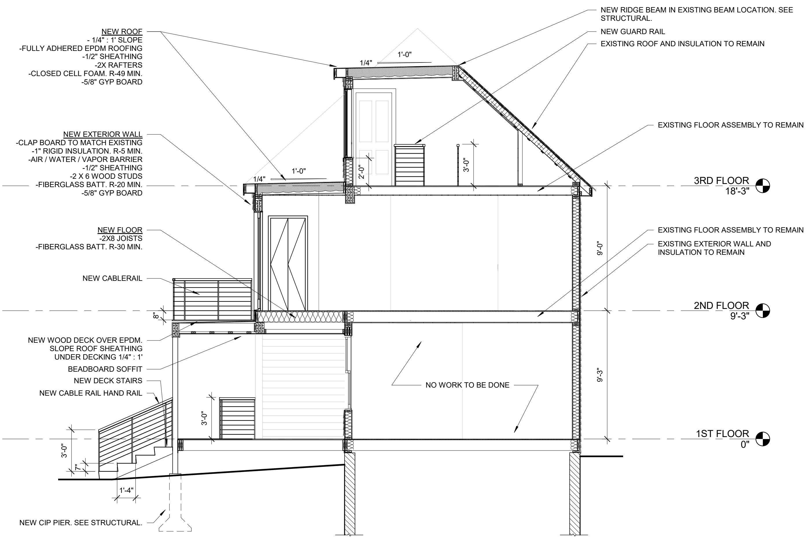
4 CROSS SECTION 1/4" = 1'-0"
