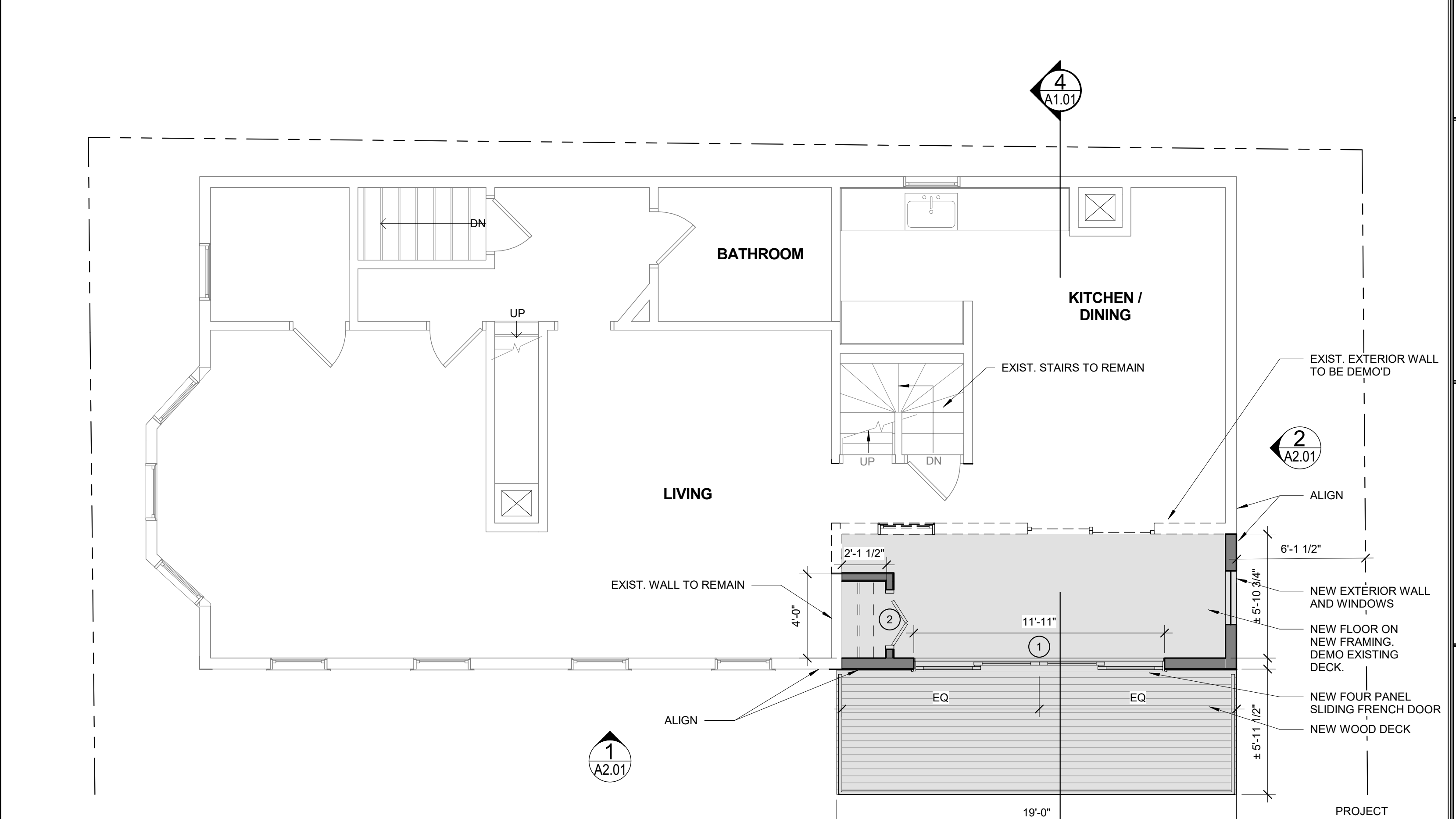
2 2ND FLOOR PLAN 1/4" = 1'-0"
