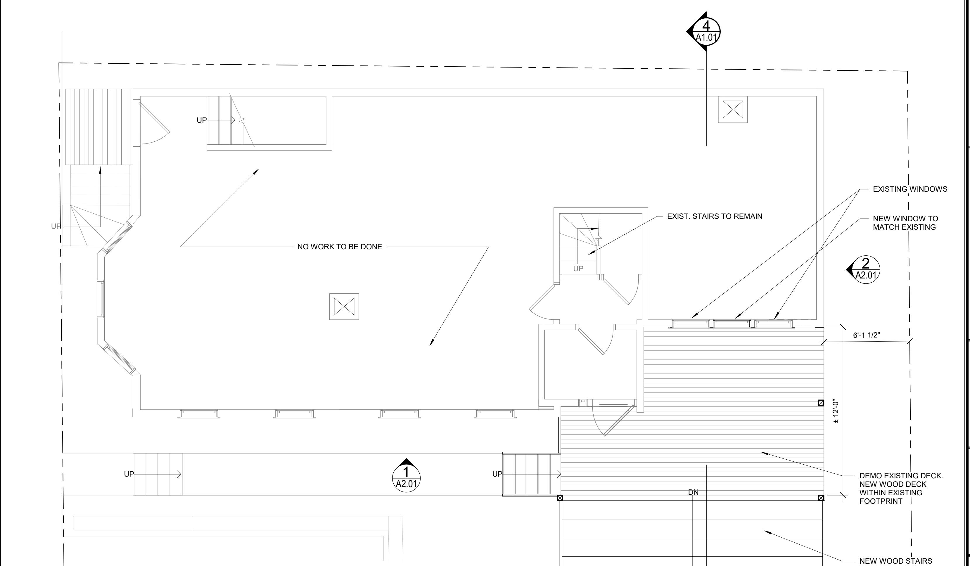
2 2ND FLOOR PLAN 1/4" = 1'-0"
