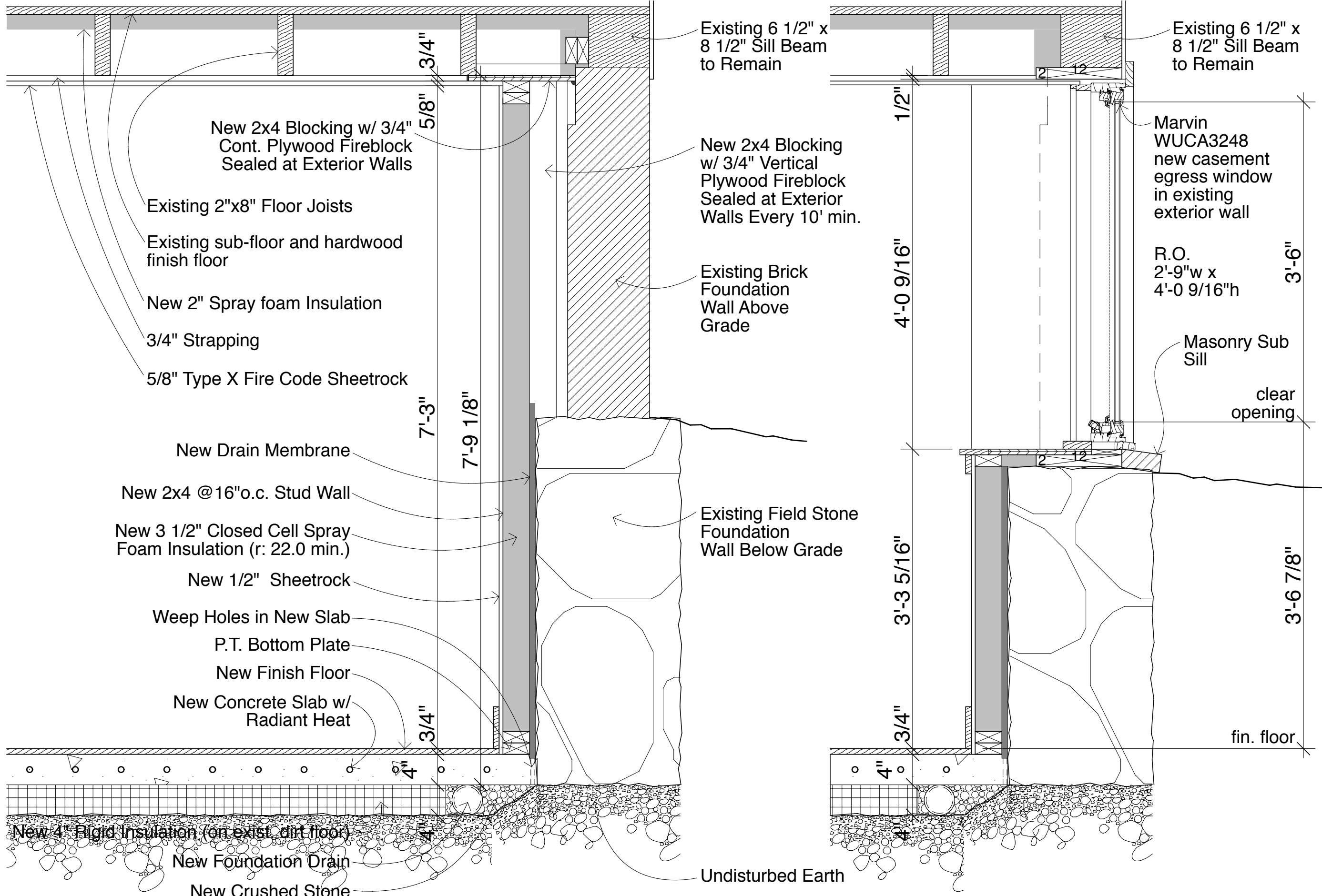
SECTION AT TYPICAL EXTERIOR WALL 0 1' 2' 4'
