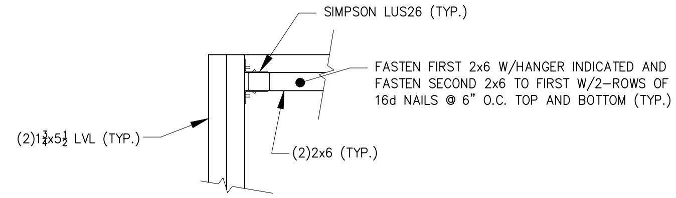
DETAIL C 1 1/2" = 1'-0"
