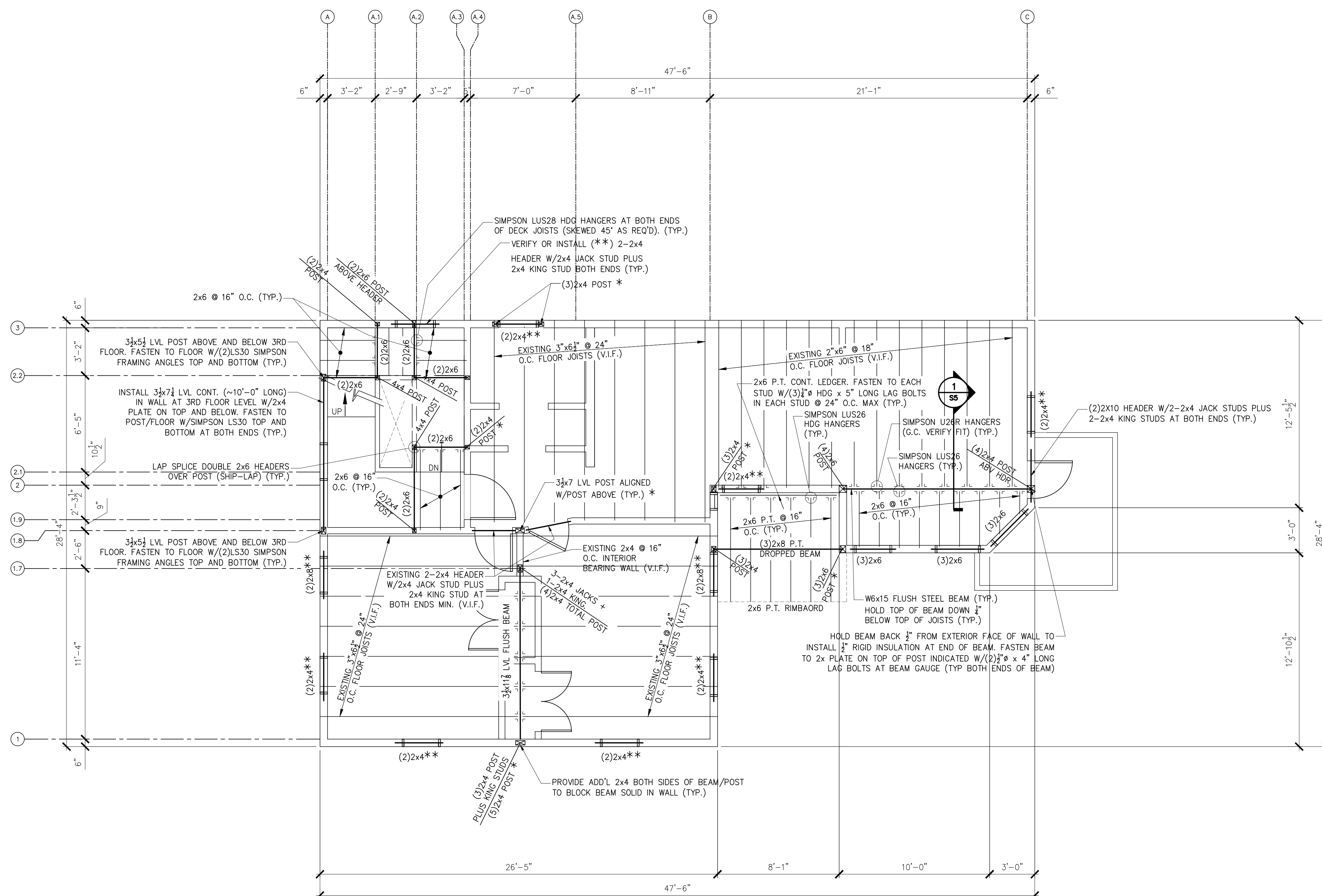
THIRD FLOOR FRAMING PLAN 1/4" = 1'-0"
