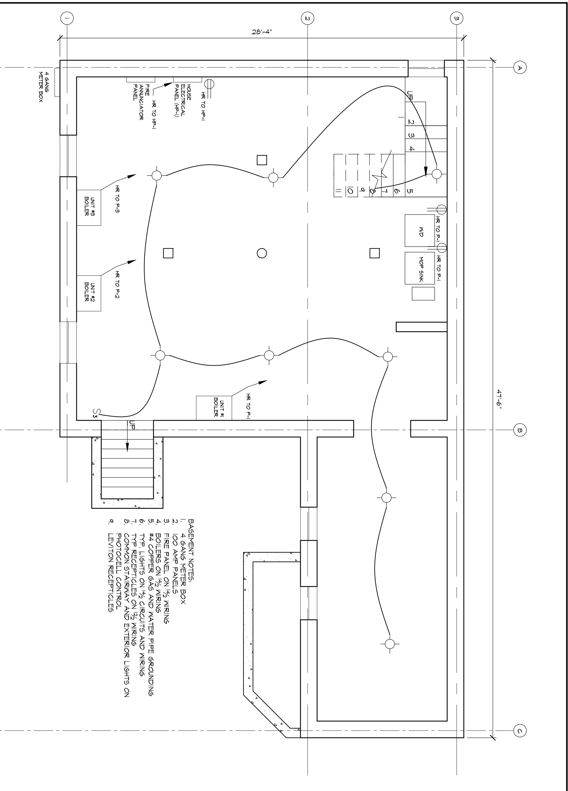
1 BASEMENT ELECTRICAL PLAN SCALE = 1/4" = 1'-0"
