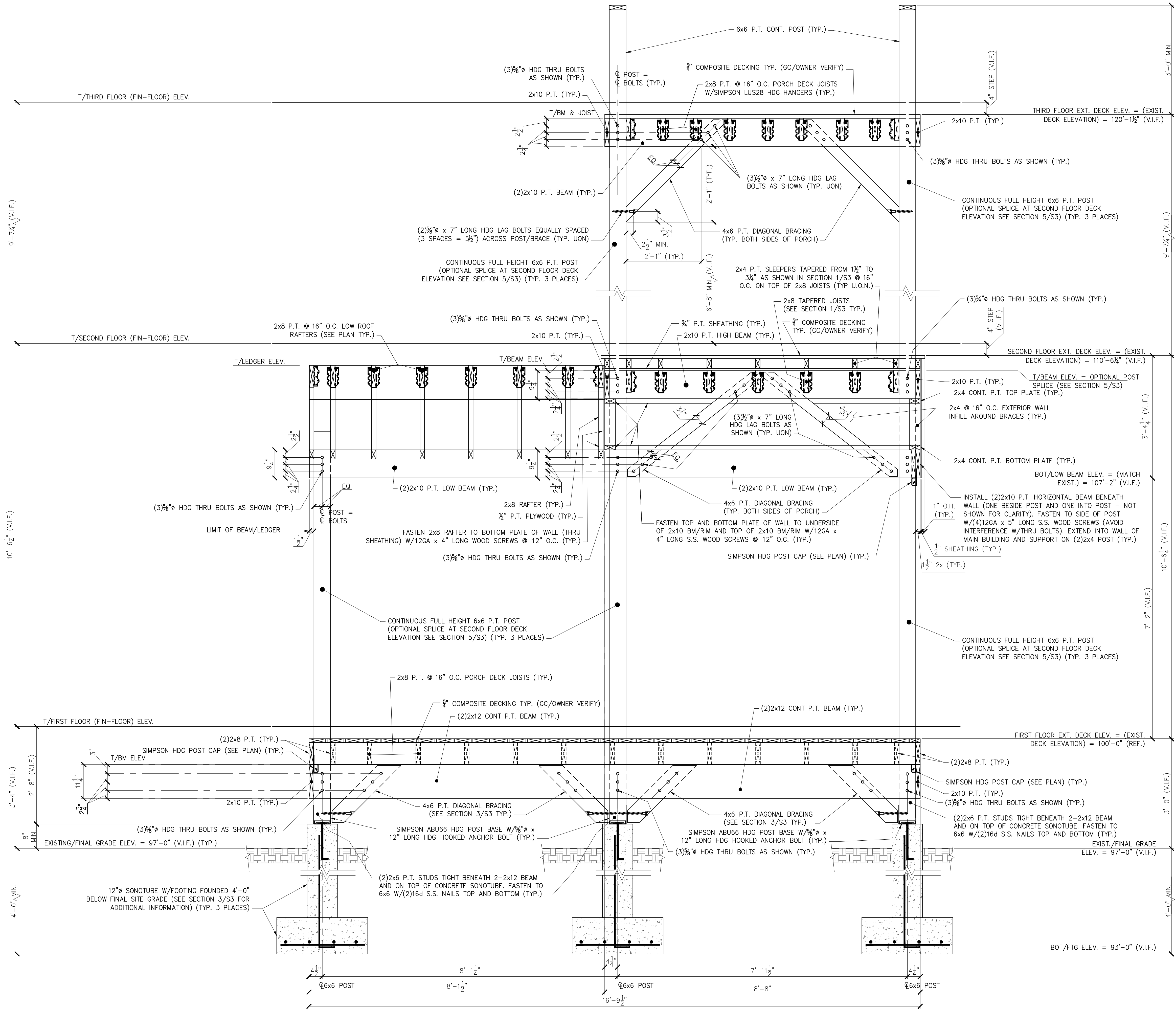
SECTION 2 3/4" = 1'-0"
