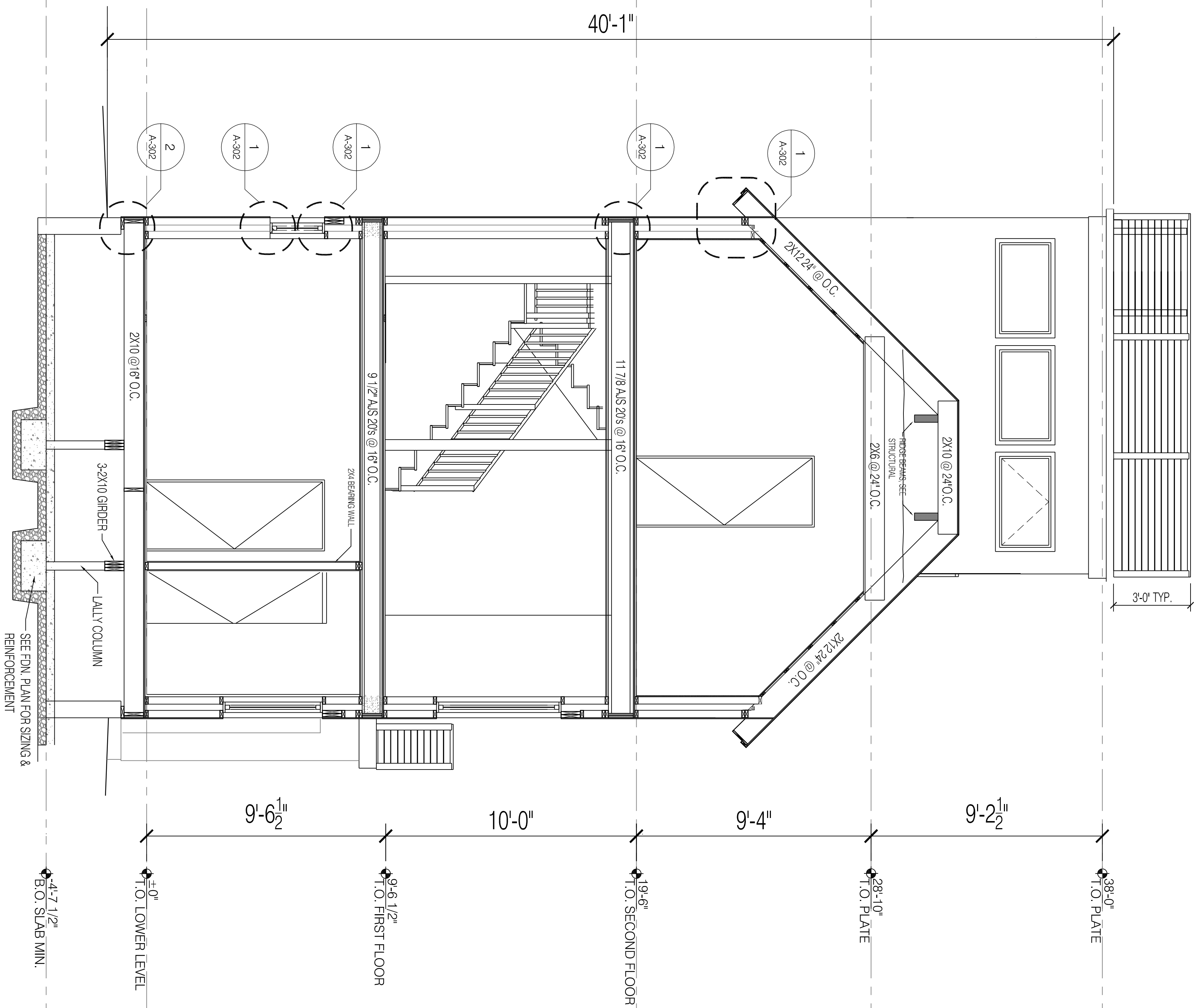
1 BUILDING SECTION 1/8" = 1'-0"
