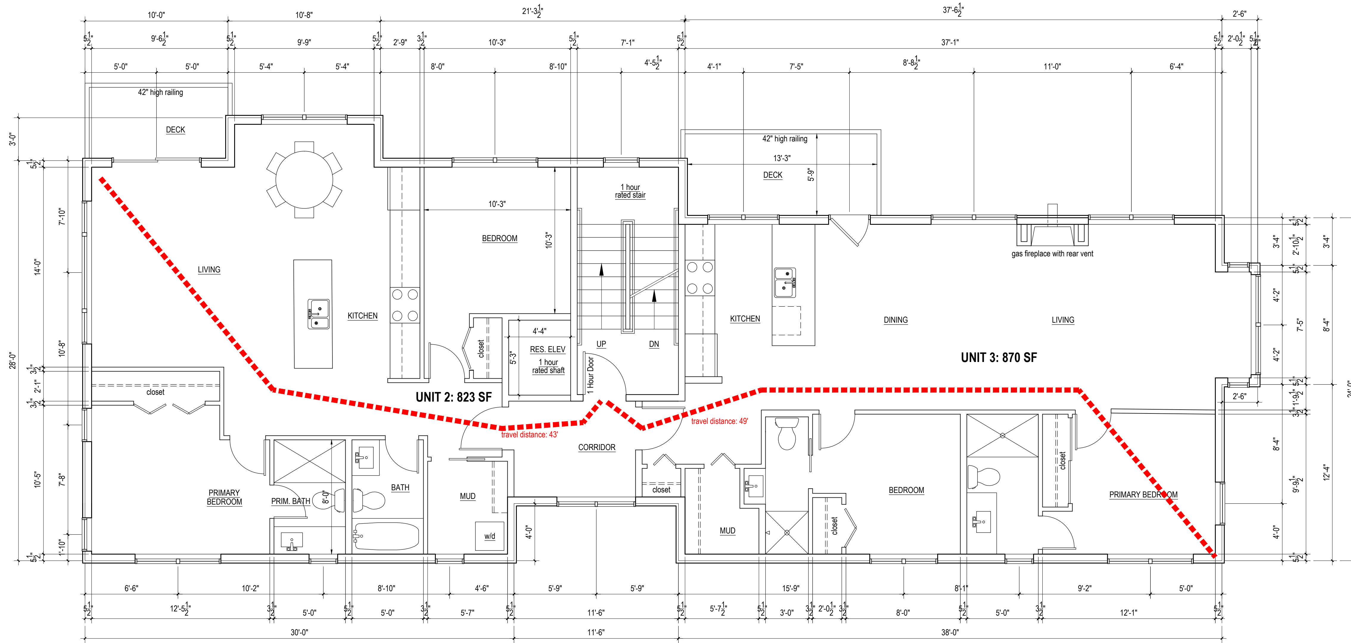
1 2nd Floor Plan 1/4" = 1'-0"
