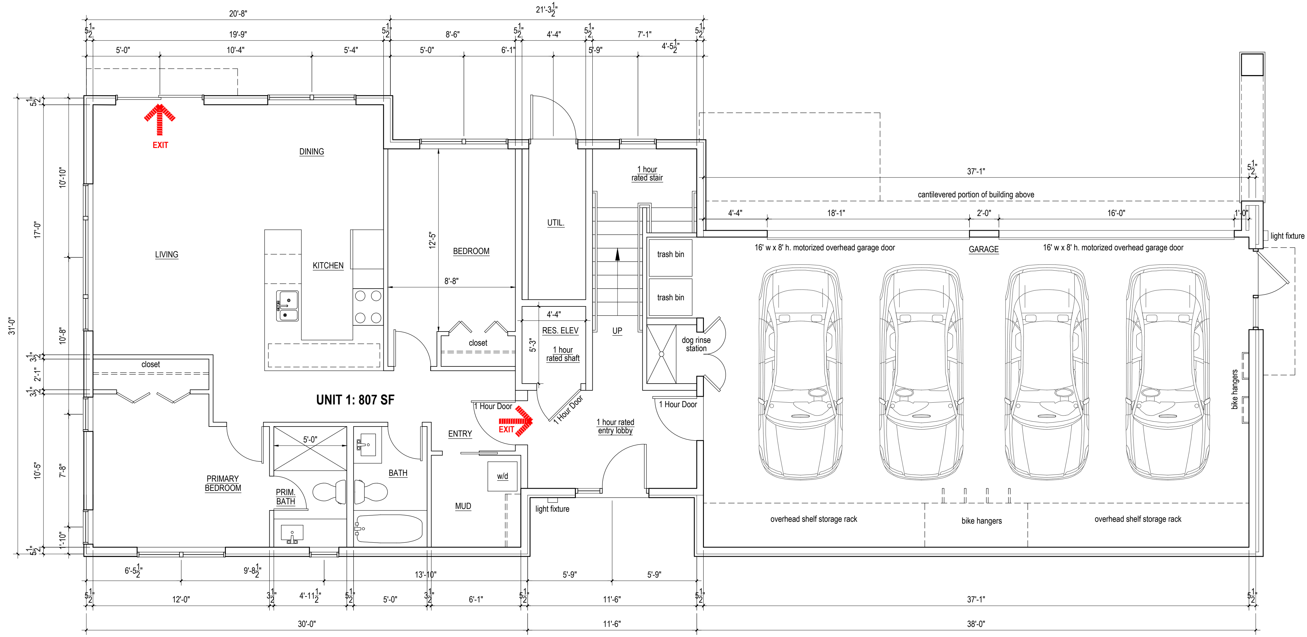
1 1st Floor Plan 1/4" = 1'-0"
