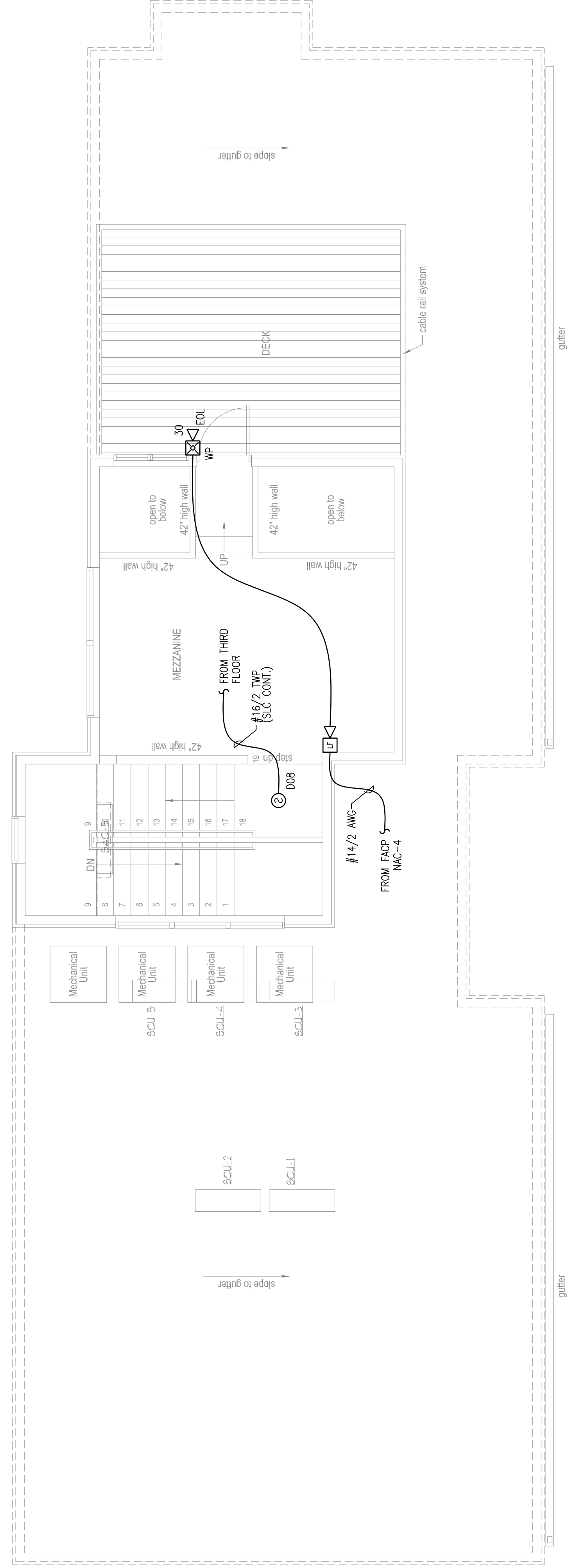
ROOF/MEZZANINE FIRE ALARM PLAN SCALE: 1/4"=1'-0"
