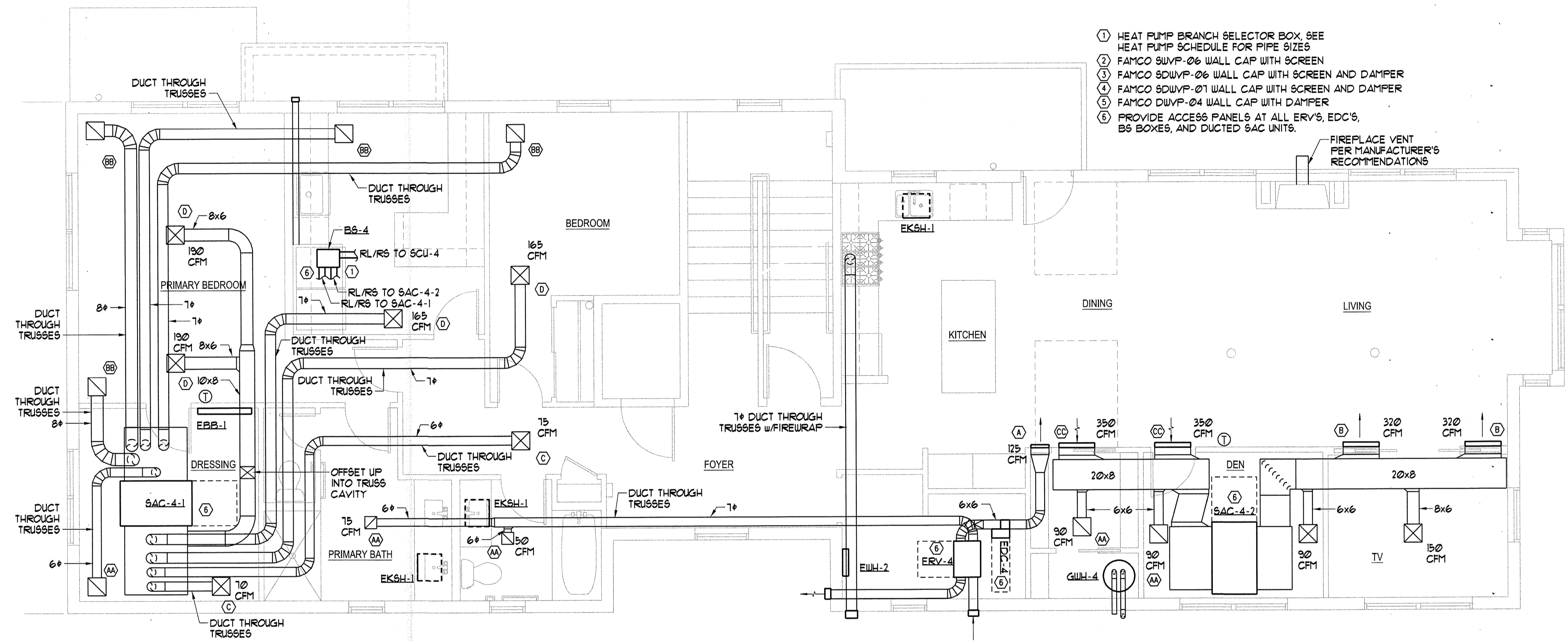
THIRD FLOOR MECHANICAL PLAN SCALE - 1/4" = 1'-0"
