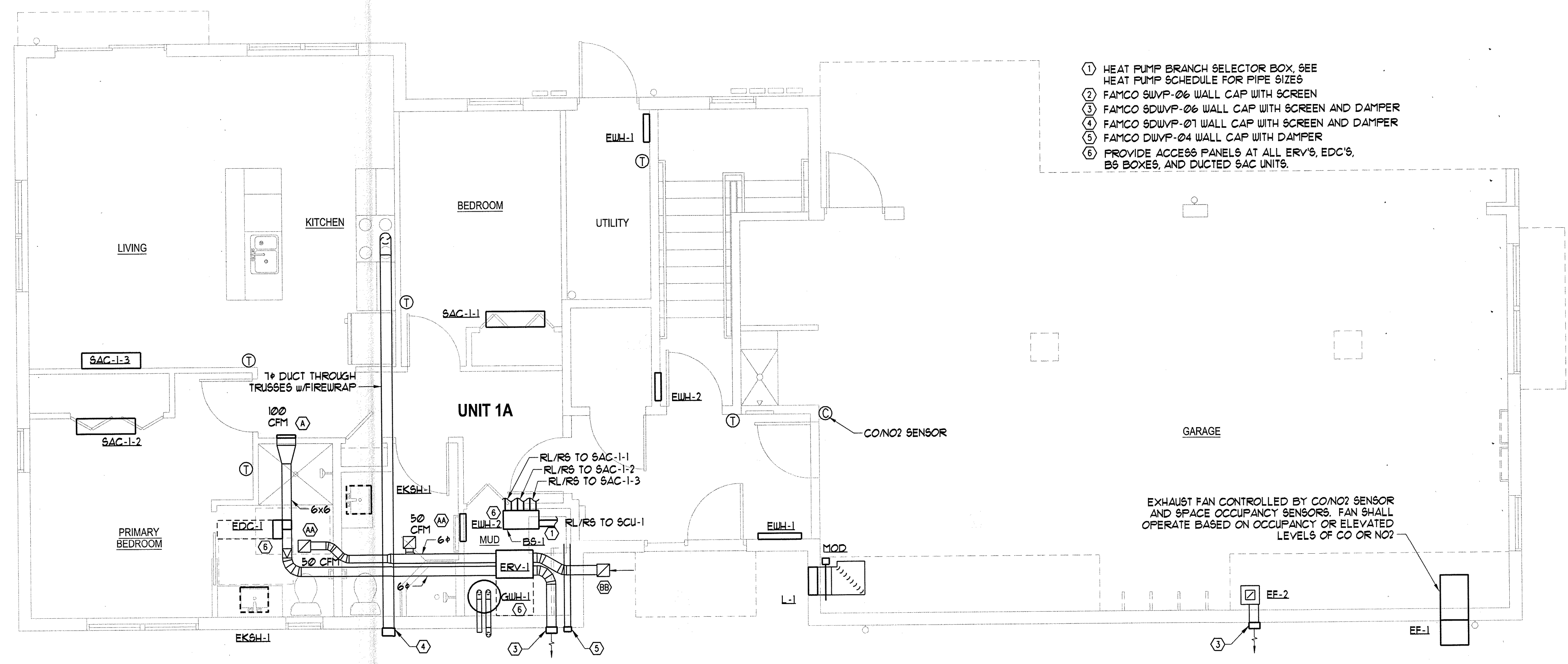
FIRST FLOOR MECHANICAL PLAN SCALE - 1/4" = 1'-0"
