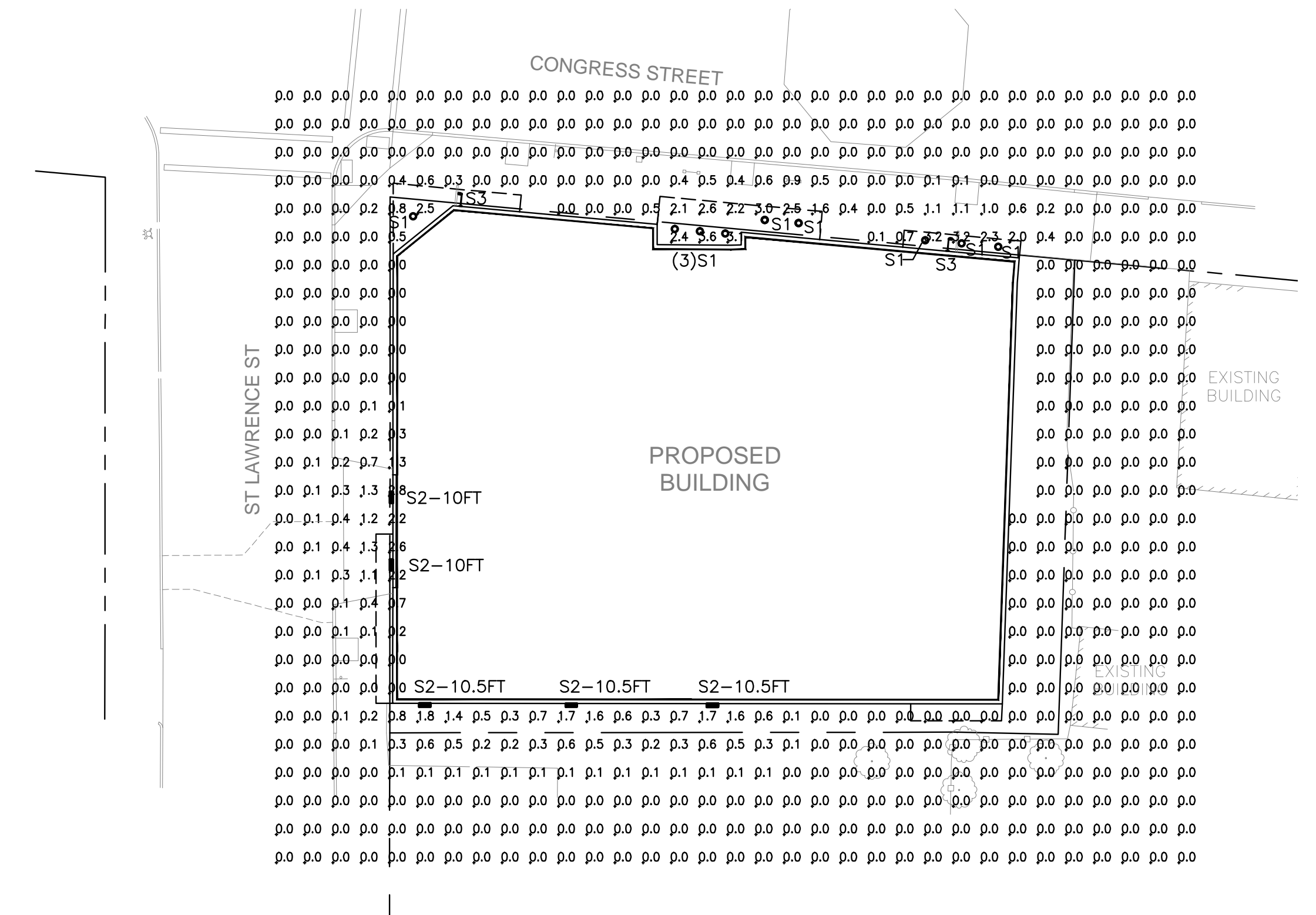
PHOTOMETRIC SITE PLAN
