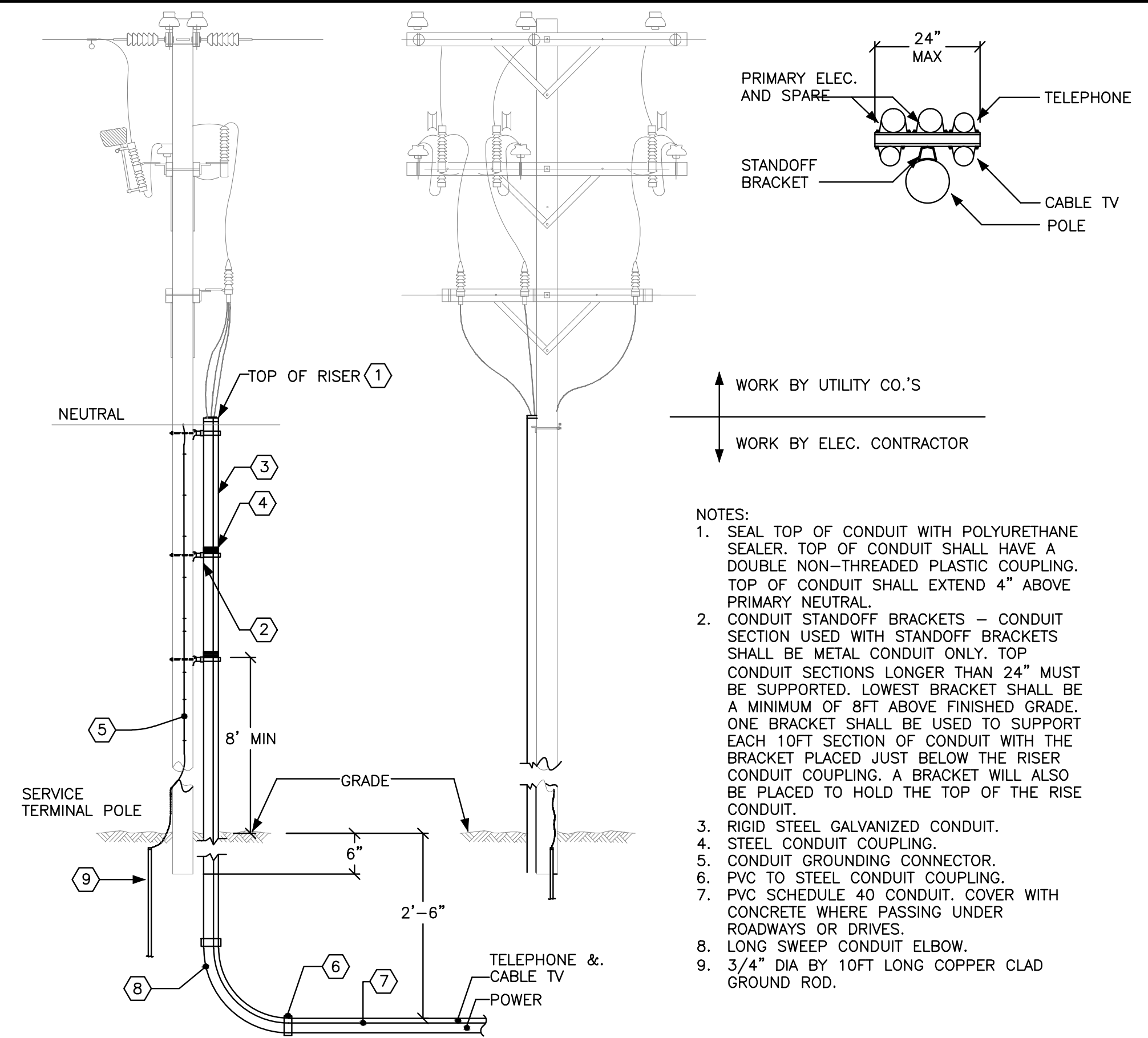
SERVICE RISER POLE DETAIL
