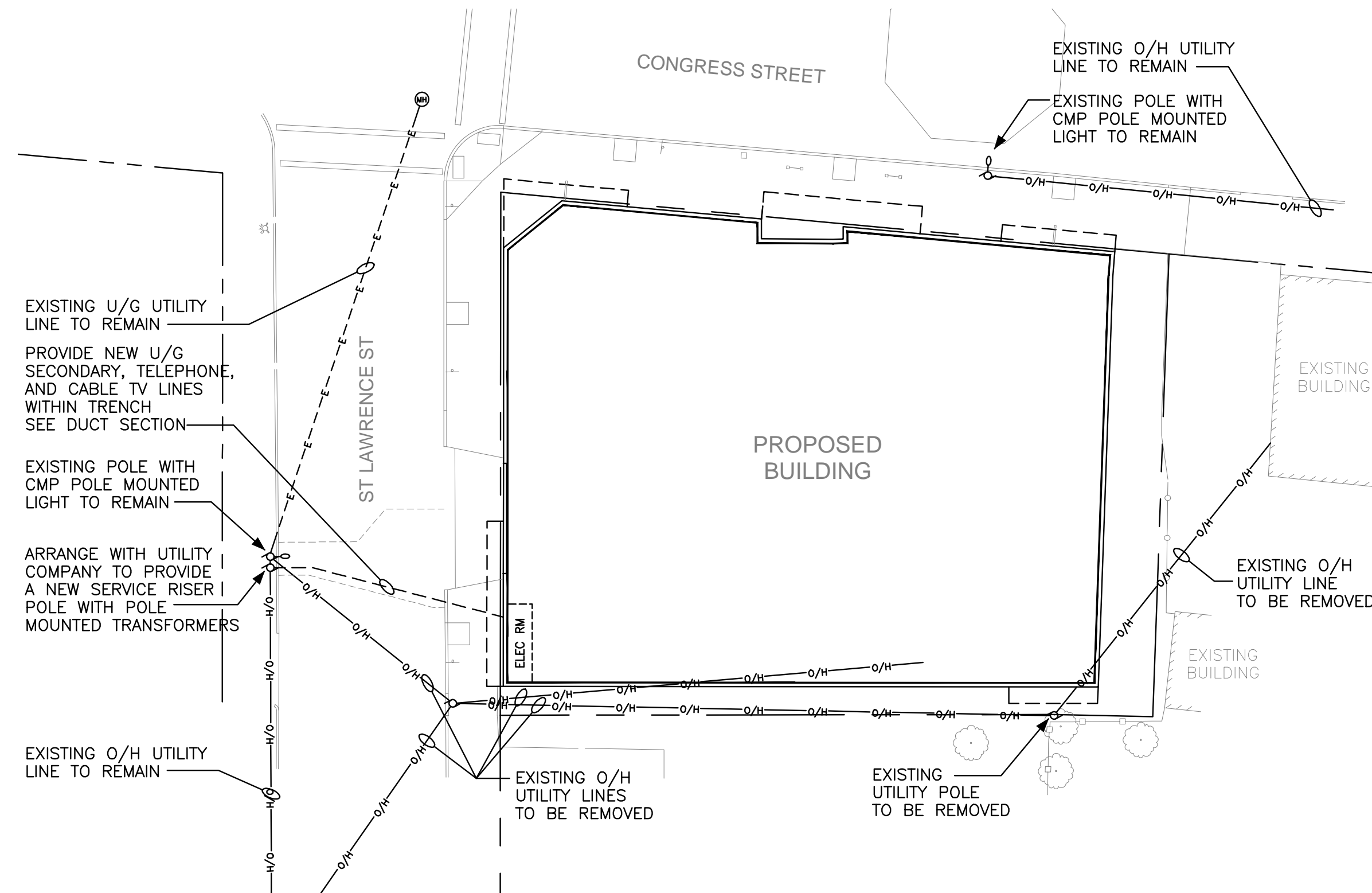
ELECTRICAL SITE PLAN
