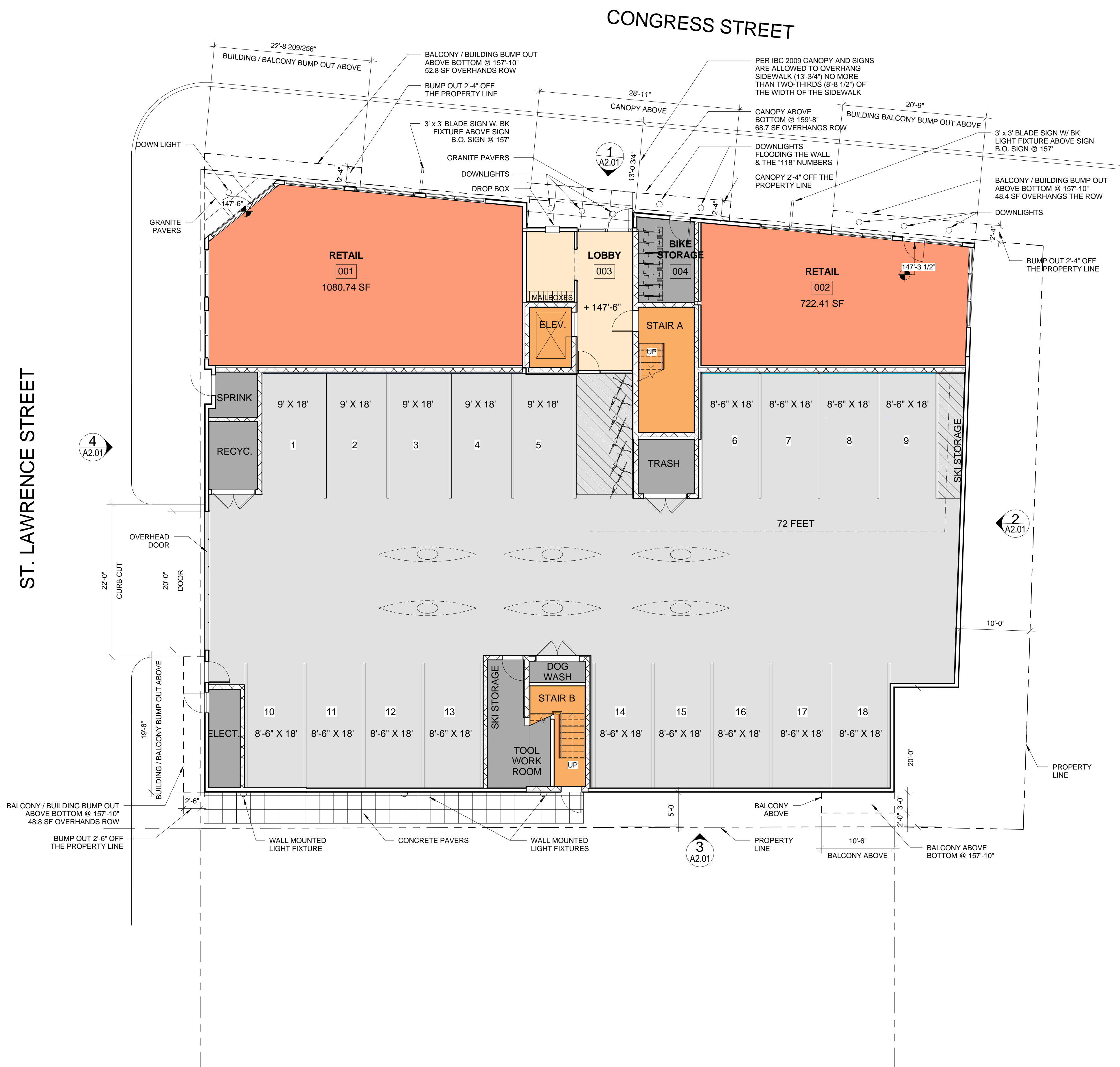
1 PARKING LEVEL PROJECT FOOTPRINT: 8,981 GSF 1/8" = 1'-0"
