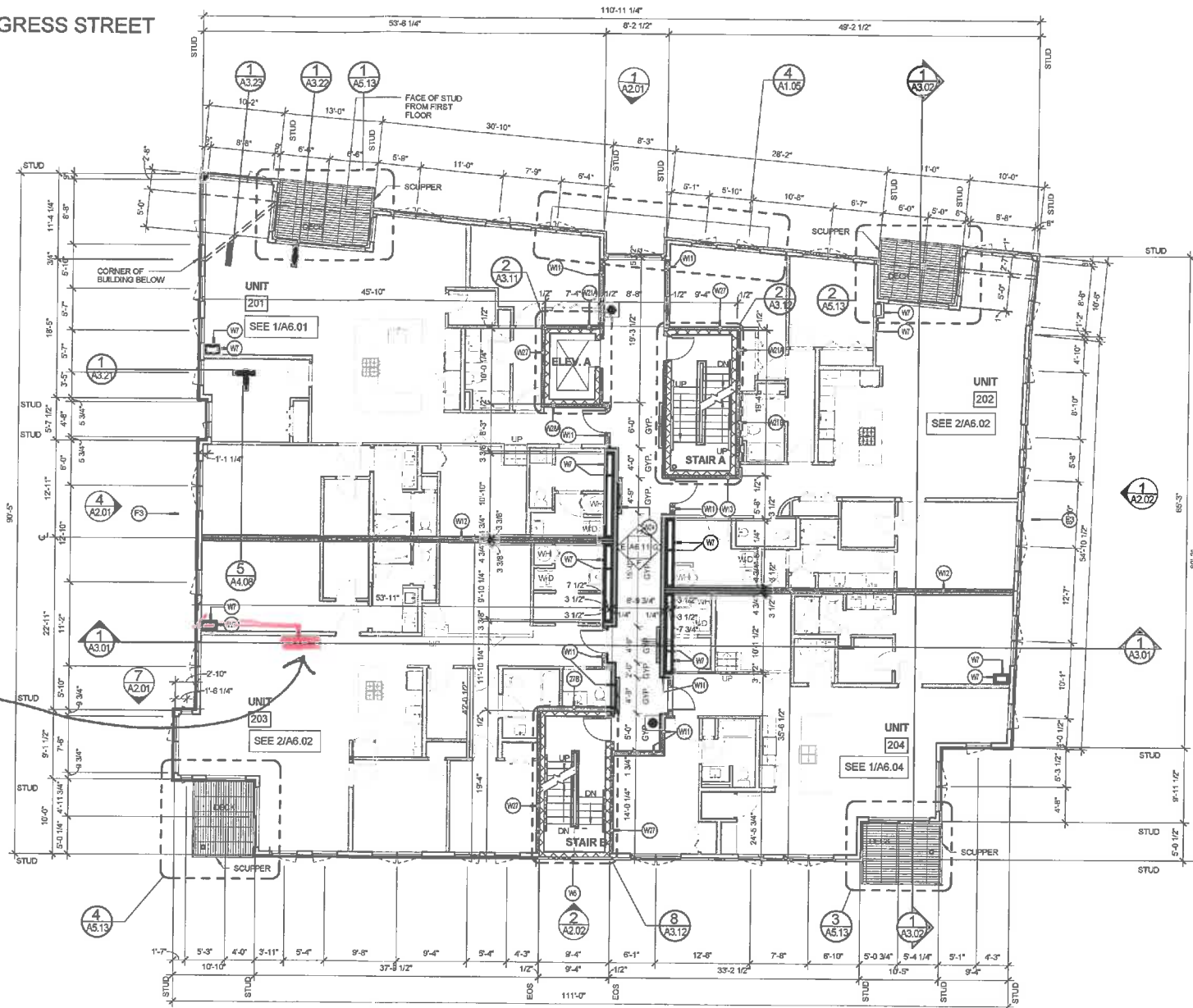
1 SECOND FLOOR PLAN 1/8" = 1'-0"
