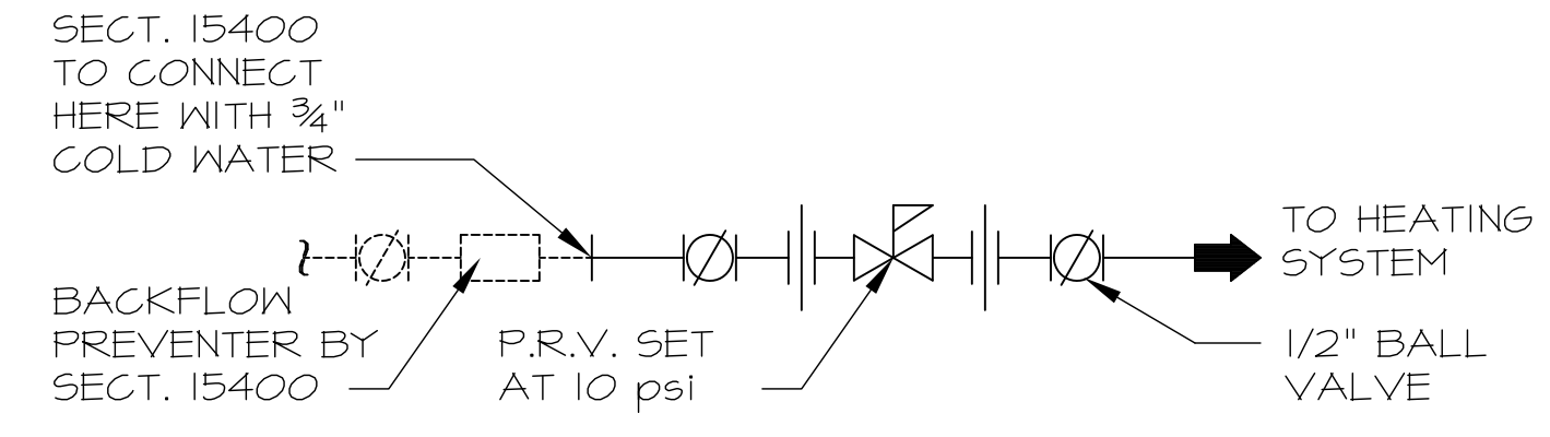
2 HEATING SYSTEM WATER MAKE-UP DETAIL NO SCALE
