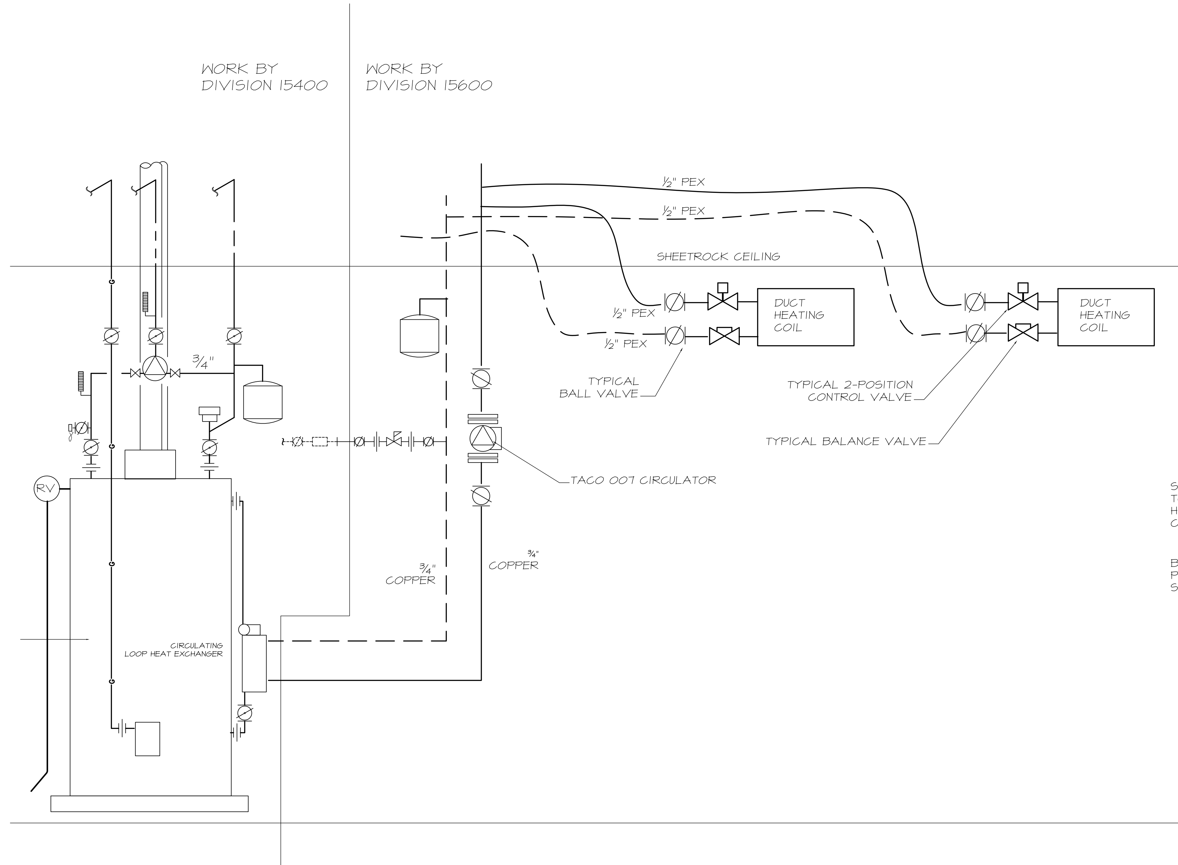
1 TYPICAL CONDOMINIUM HEATING DETAIL NO SCALE
