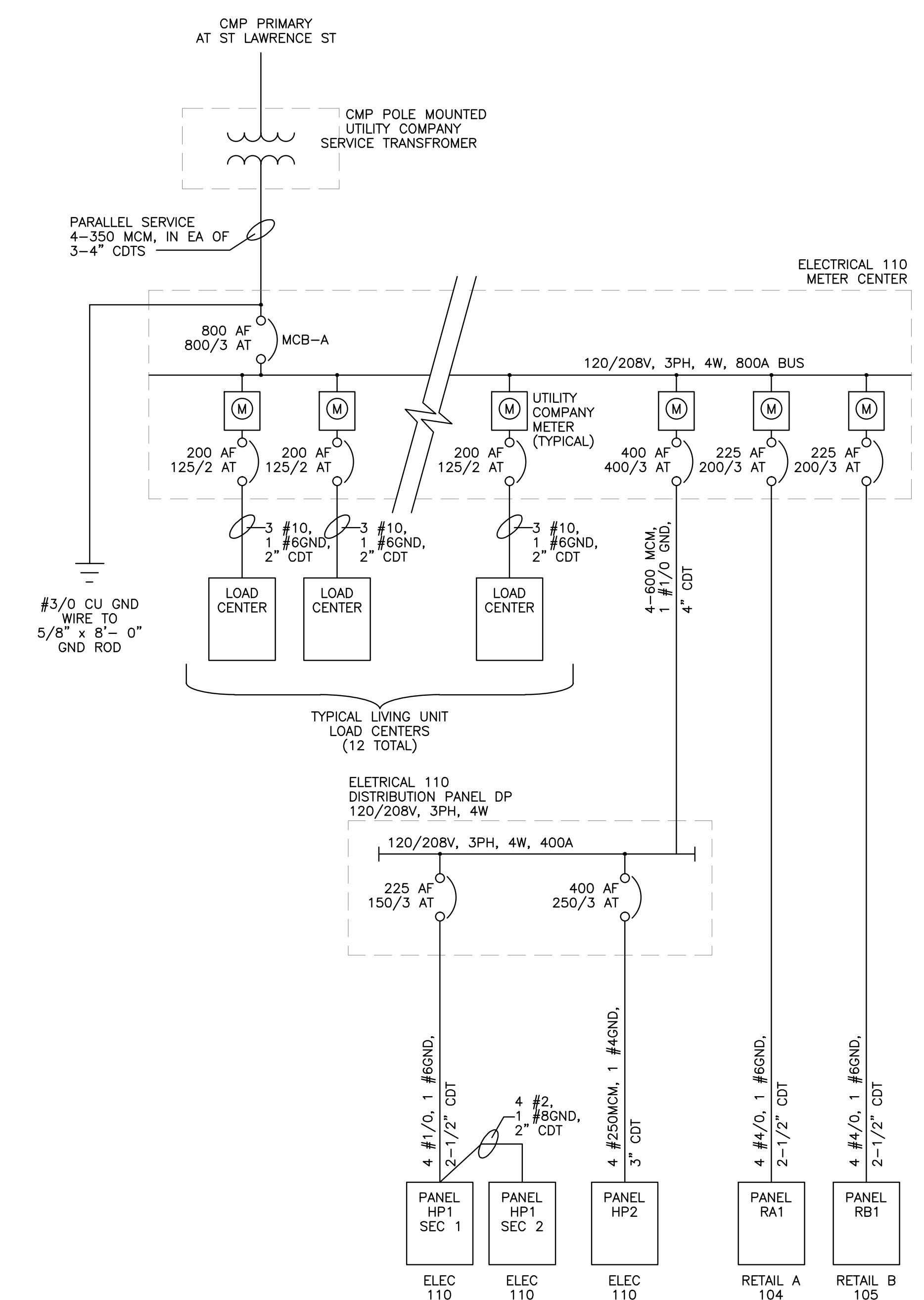
SINGLE LINE RISER DIAGRAM NOT TO SCALE
