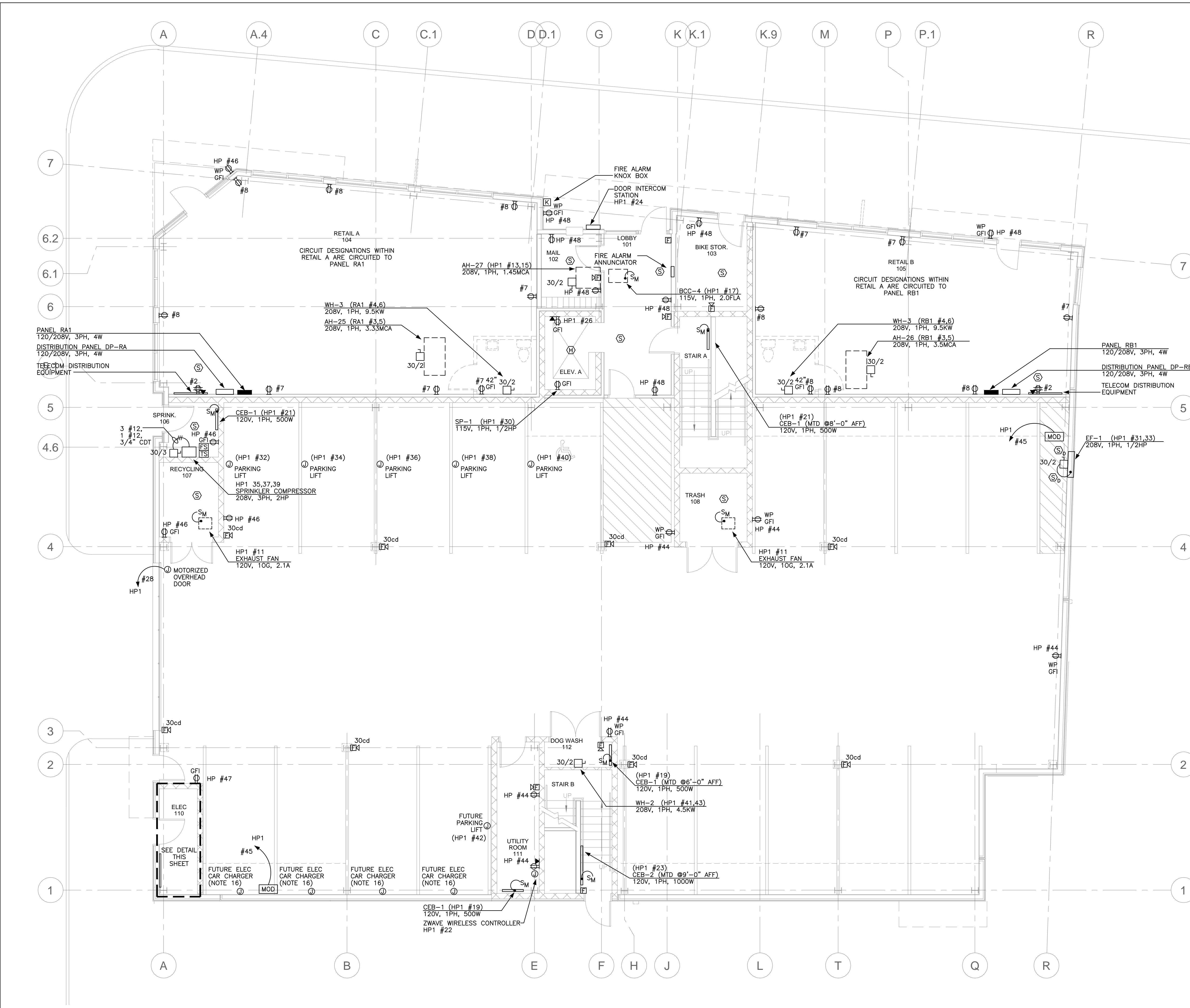
ELECTRICAL 110 1/4" = 1'-0"
