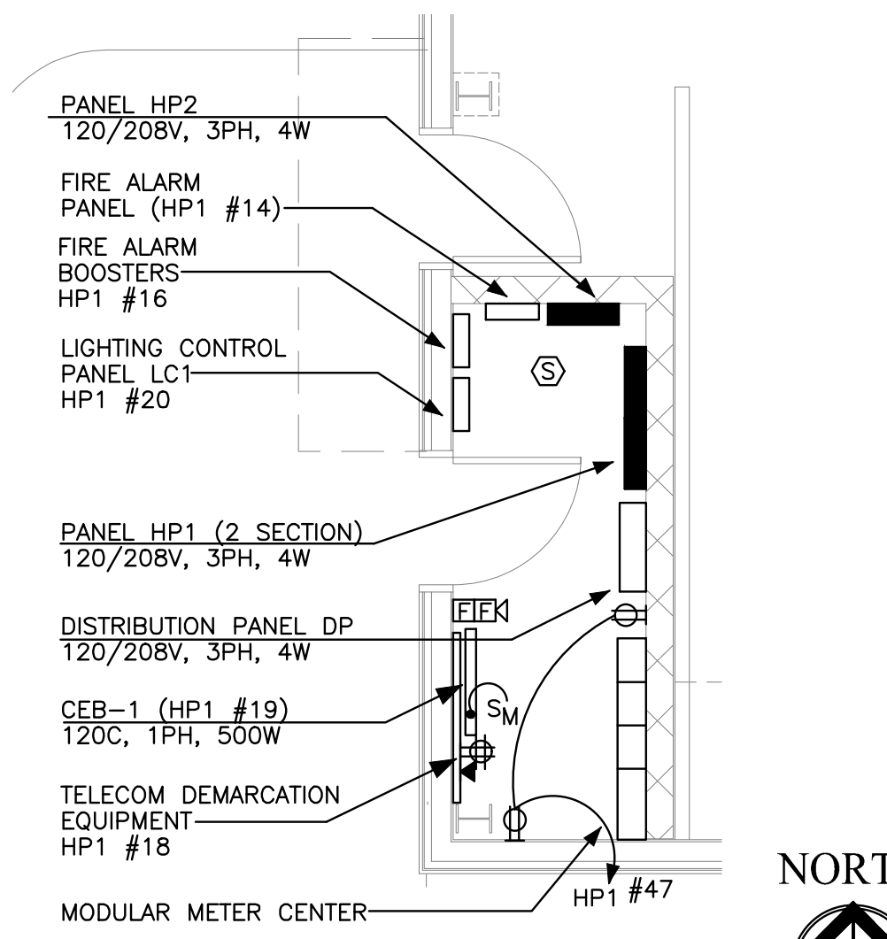
ELECTRICAL 110 1/4" = 1'-0"
