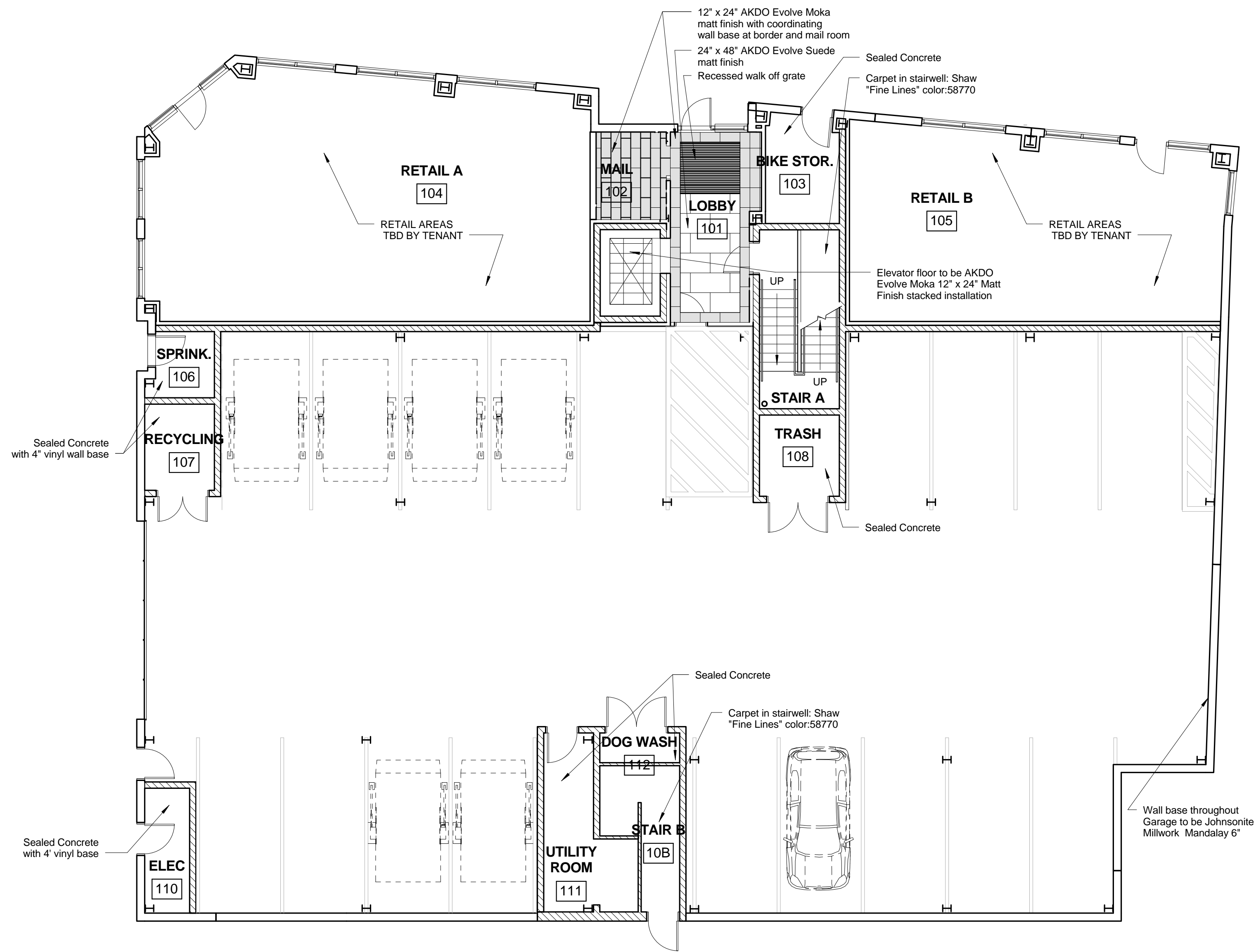
2 | 1ST FLOOR FINISH PLAN
