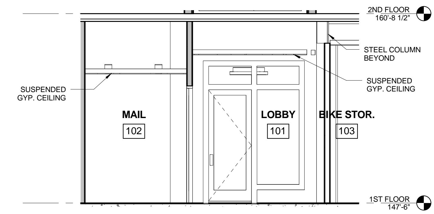
2 | SECTION AT ENTRANCE LOBBY 1/4" = 1'-0" 0 4' 8'
