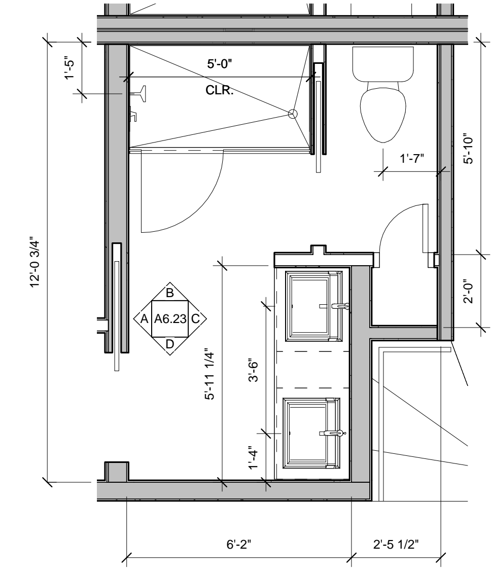
1 | UNITS 203, 303 - PRIMARY BATH PLAN
