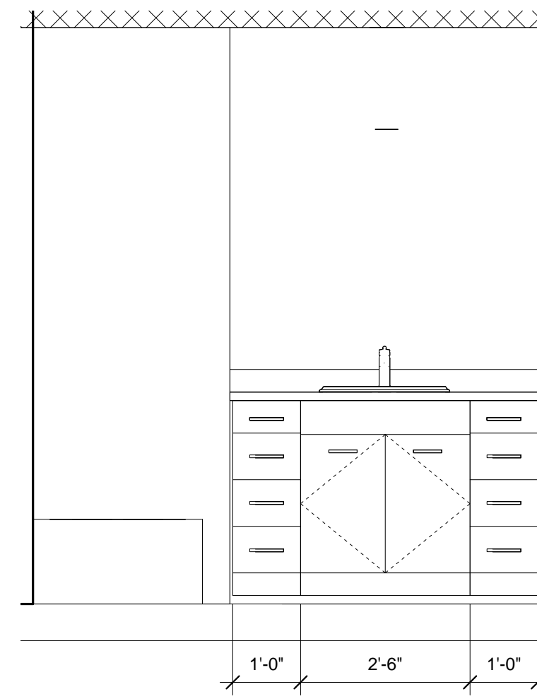
E | UNITS 203, 303 GUEST BATH ELEV. E
