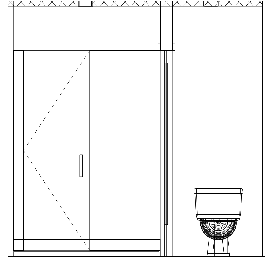
B | UNITS 203, 303 PRIMARY BATH ELEV. B
