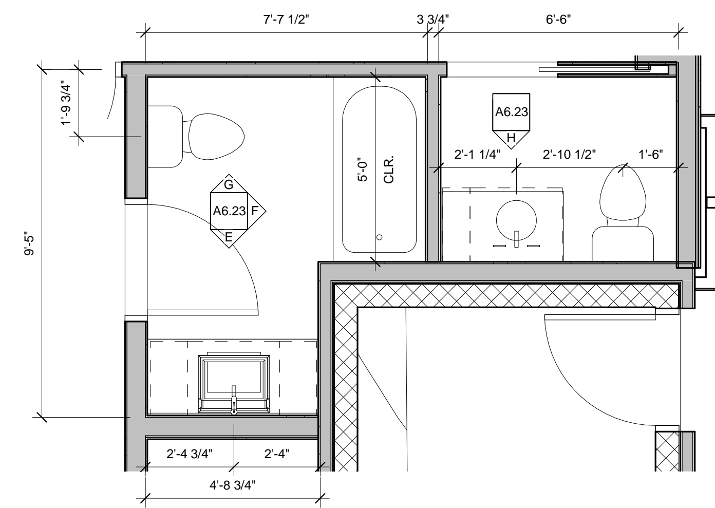
2 | UNITS 203, 303 - GUEST BATH, POWDER RM
