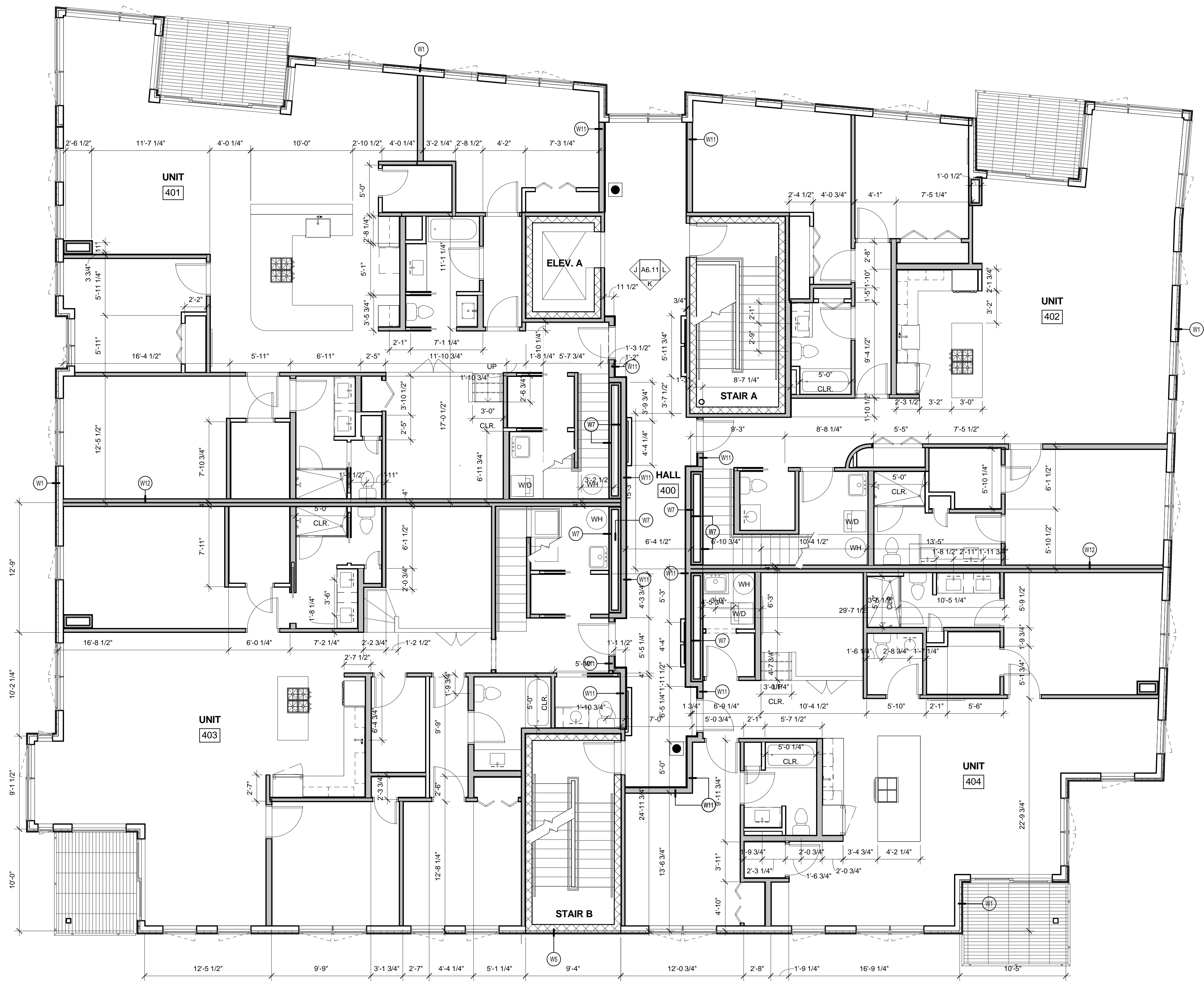
1 | 4TH FLOOR - ENLARGED PLAN 3/16" = 1'-0"
