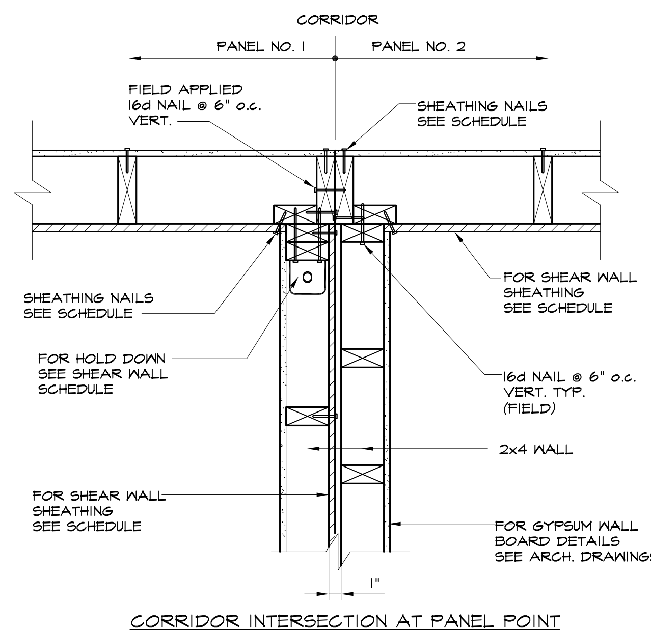
CORRIDOR INTERSECTION AT PANEL POINT
