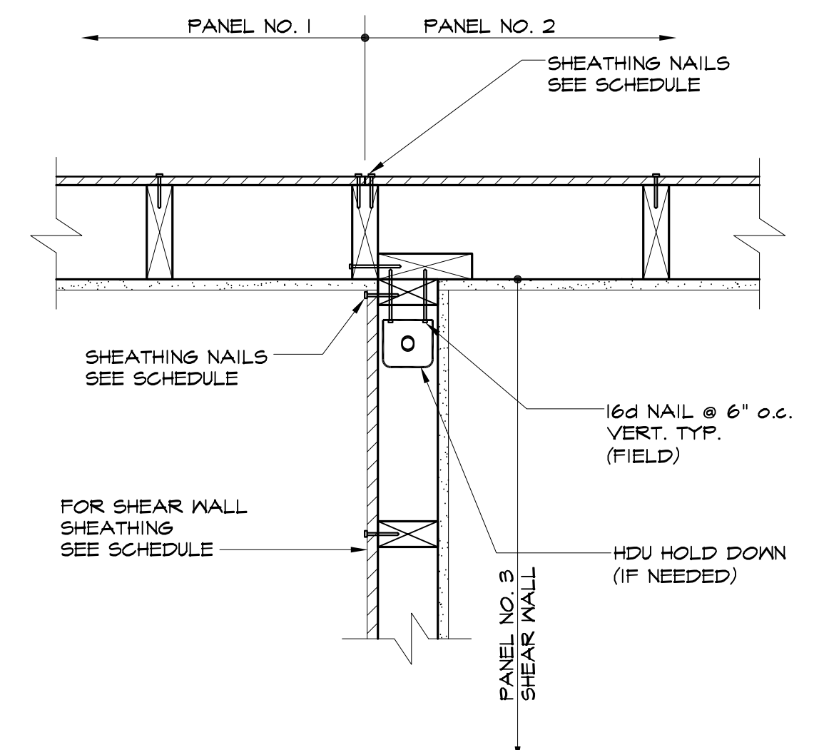
TYPICAL SHEAR WALL DETAILS AT EXTERIOR WALL
