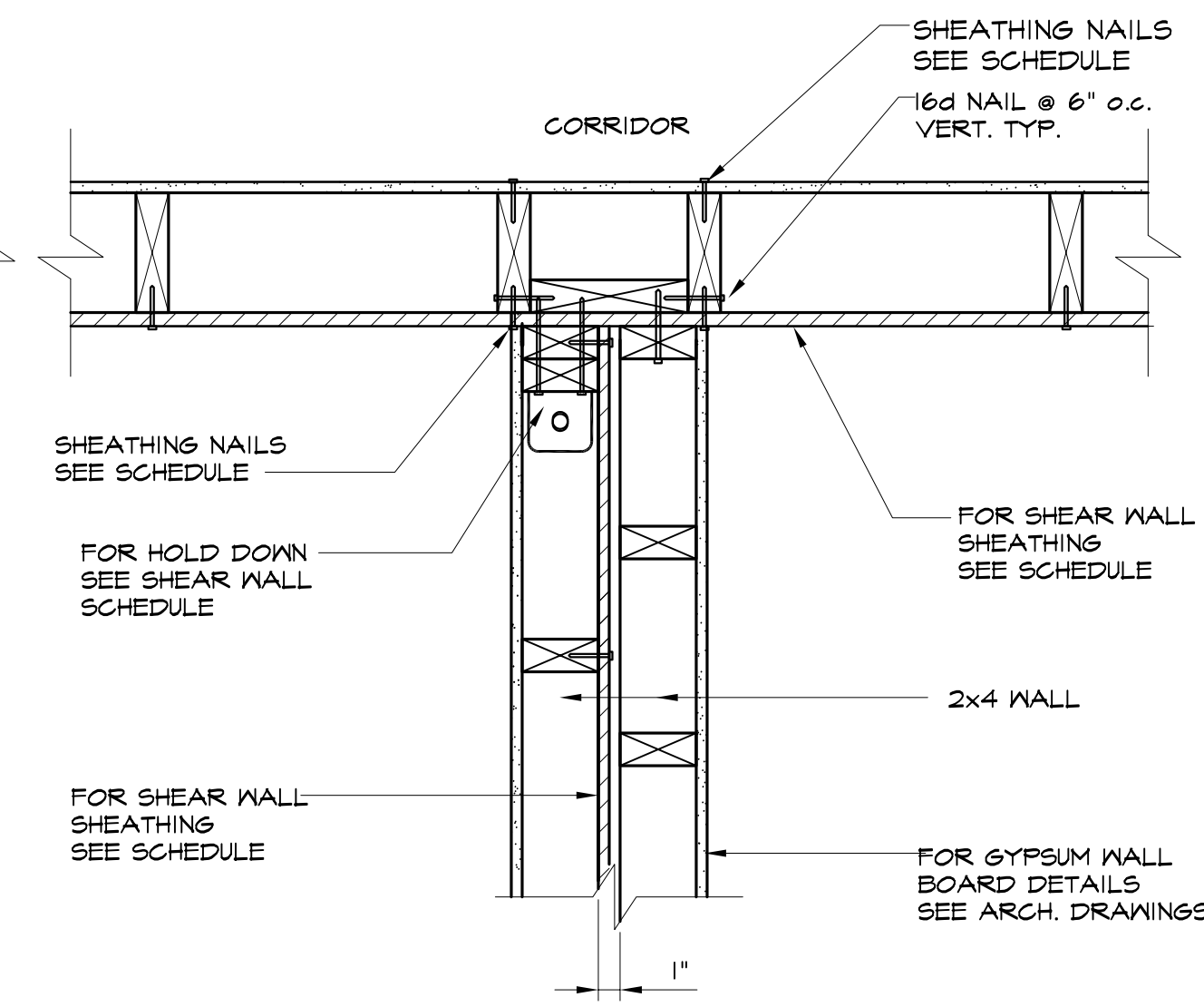
CORRIDOR INTERSECTION NOT AT PANEL POINT W/ OSB RUNNING THRU
