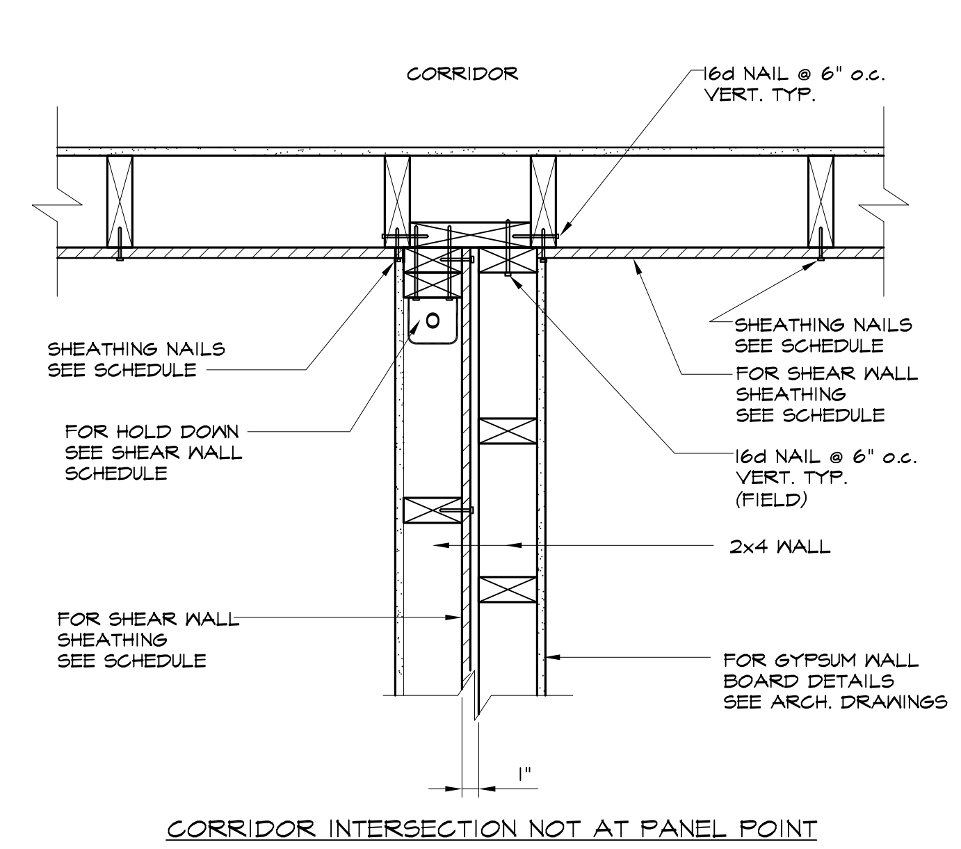
CORRIDOR INTERSECTION NOT AT PANEL POINT
