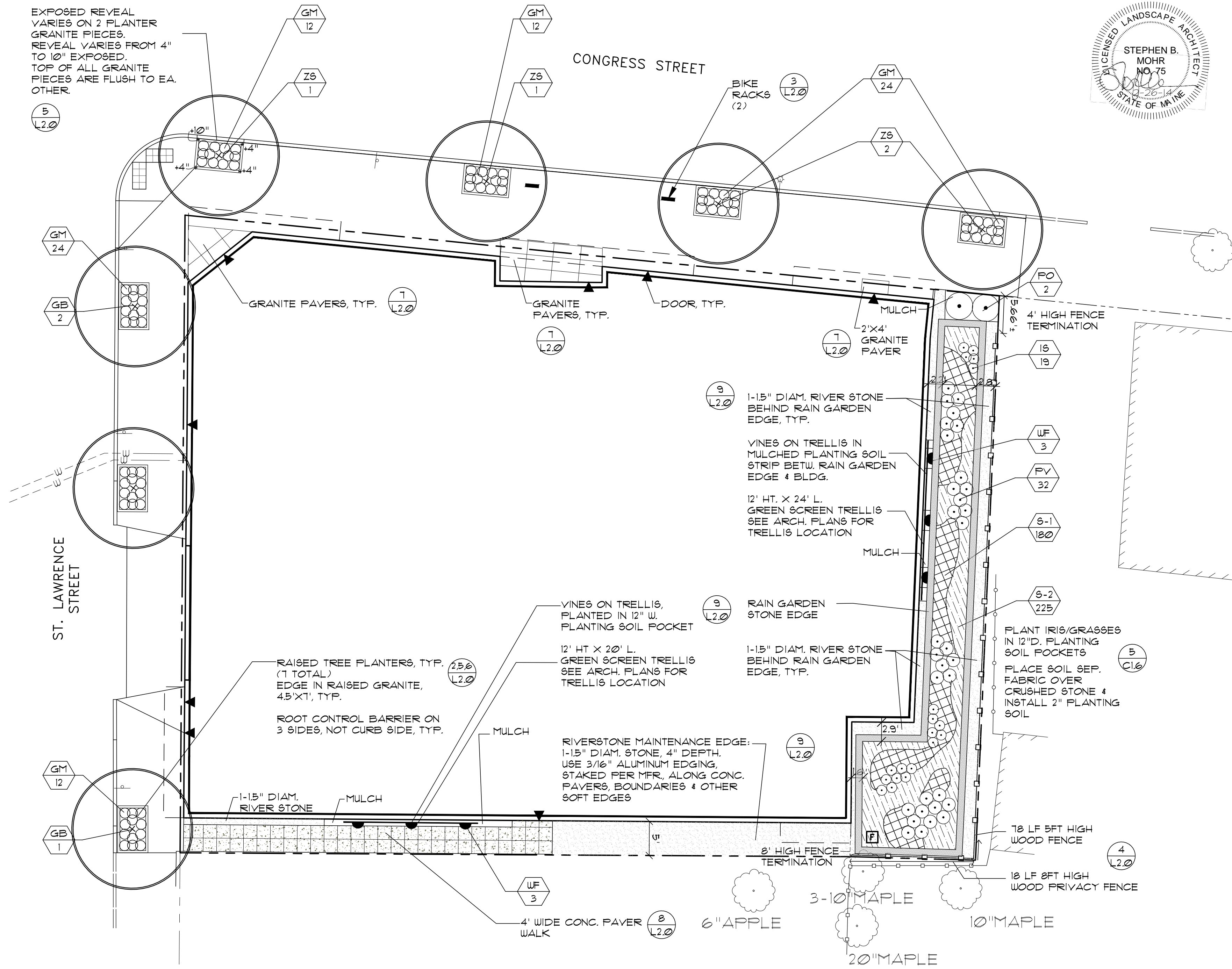
1 LANDSCAPE PLAN SCALE: 1" = 10'-0"
