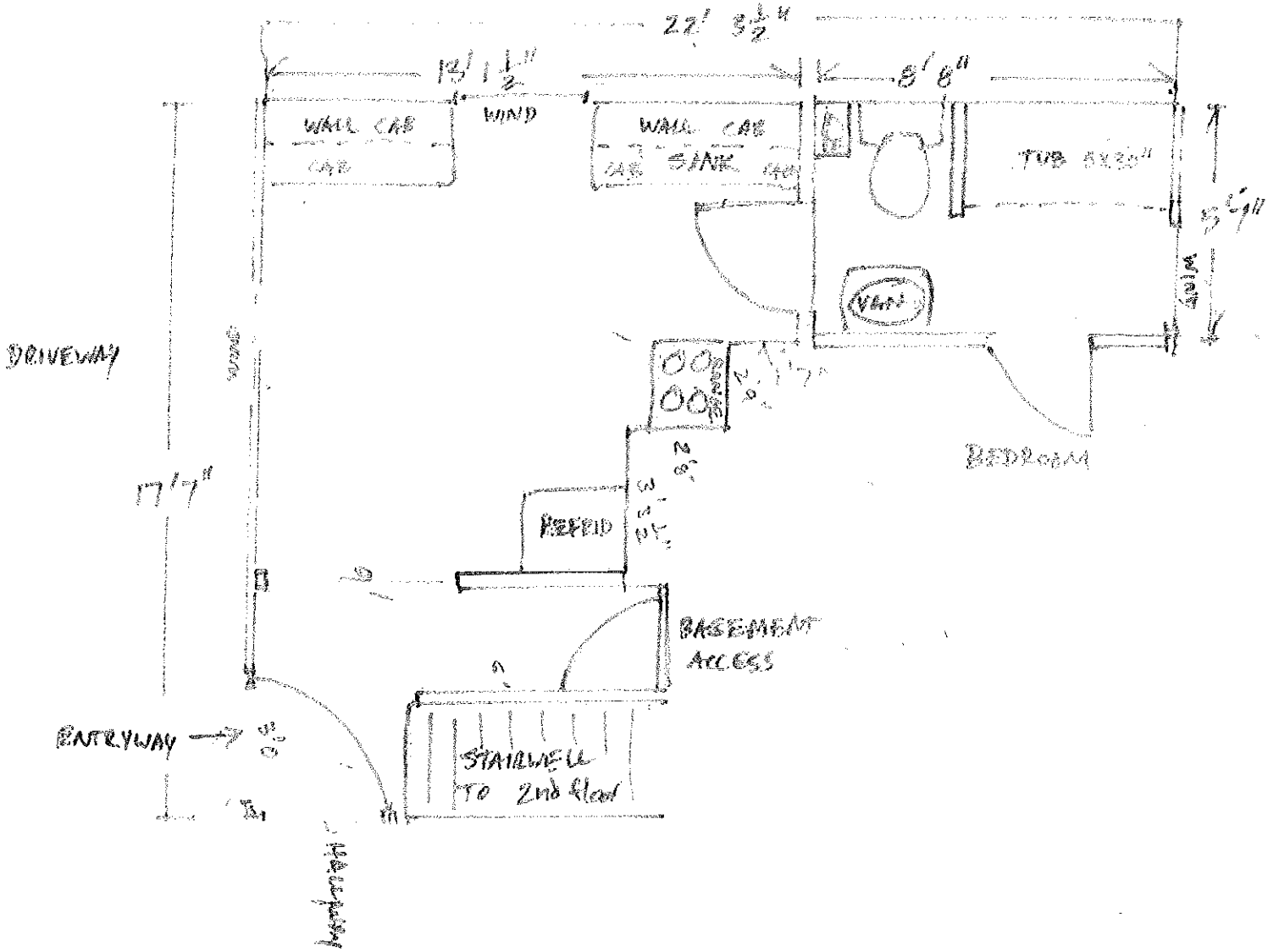
EXISTING FLOOR PLAN SCALE = 1/4" = 1'0"
