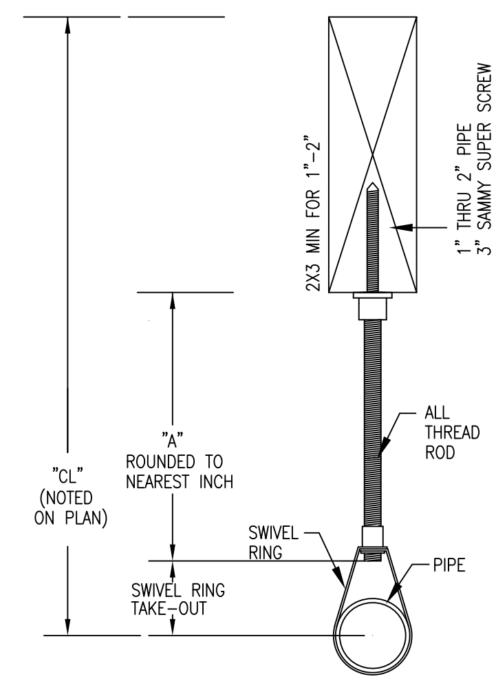
TYPE 'P' HANGER NO SCALE
