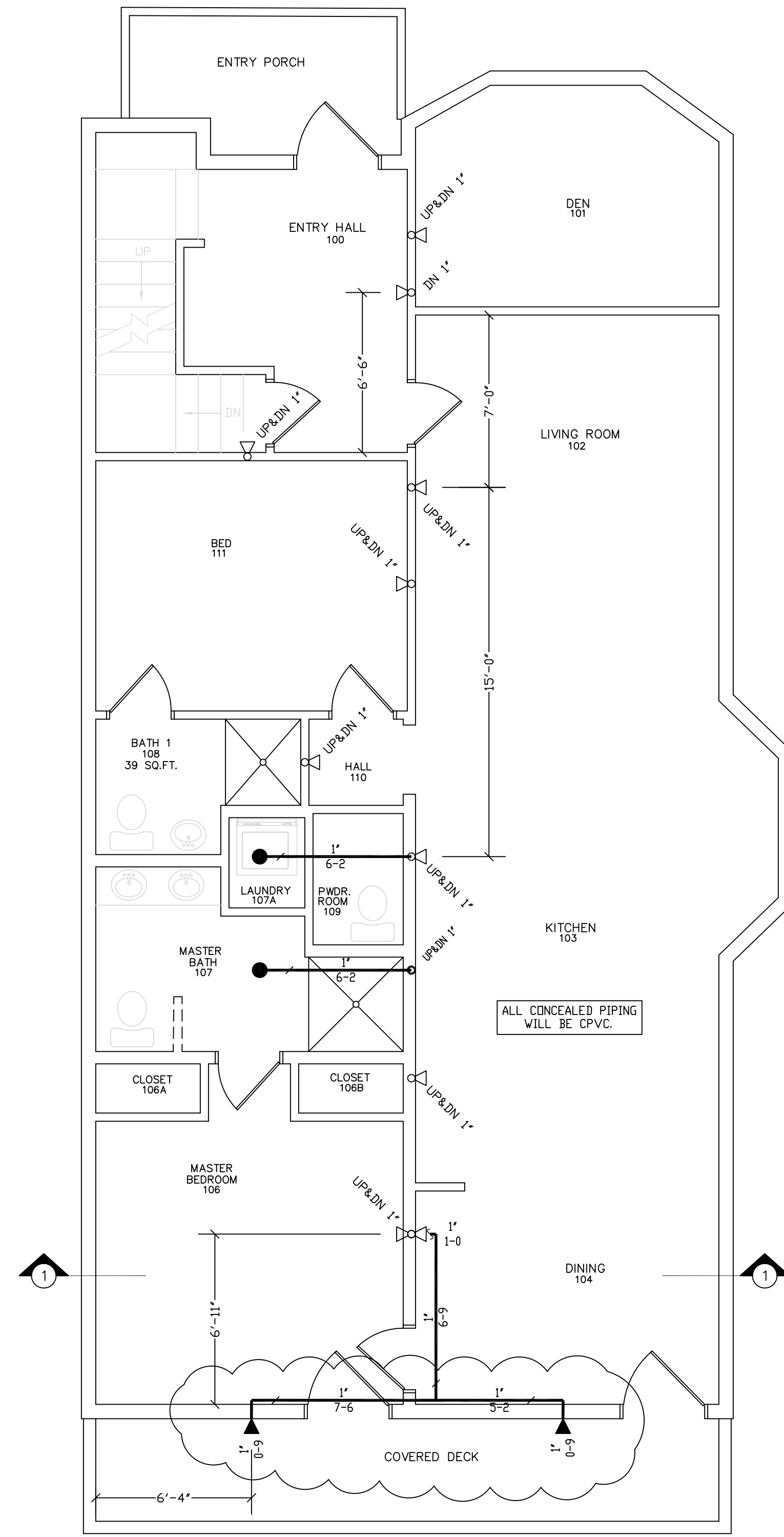
GROUND FLOOR FIRE PROTECTION
