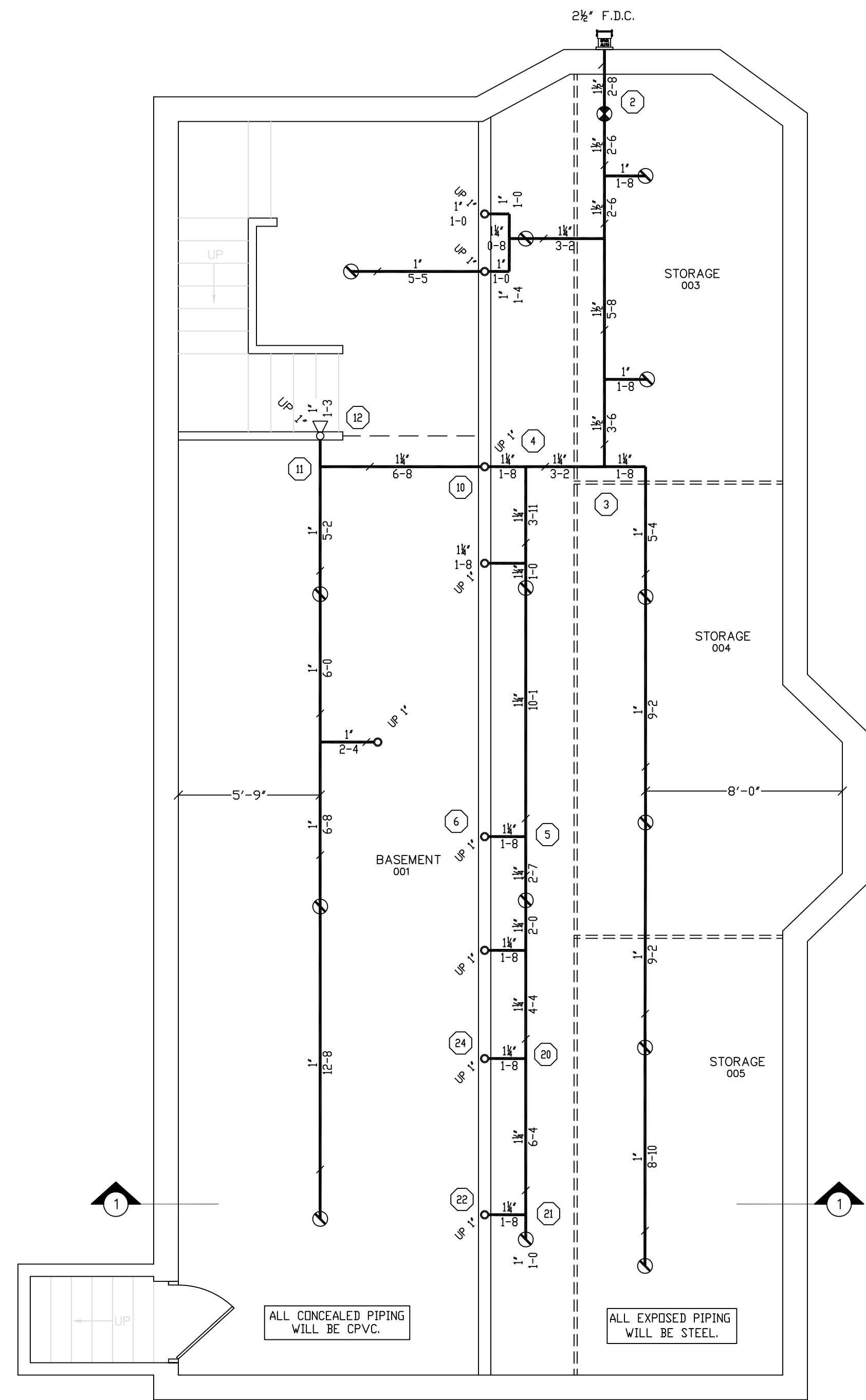
BASEMENT FIRE PROTECTION
