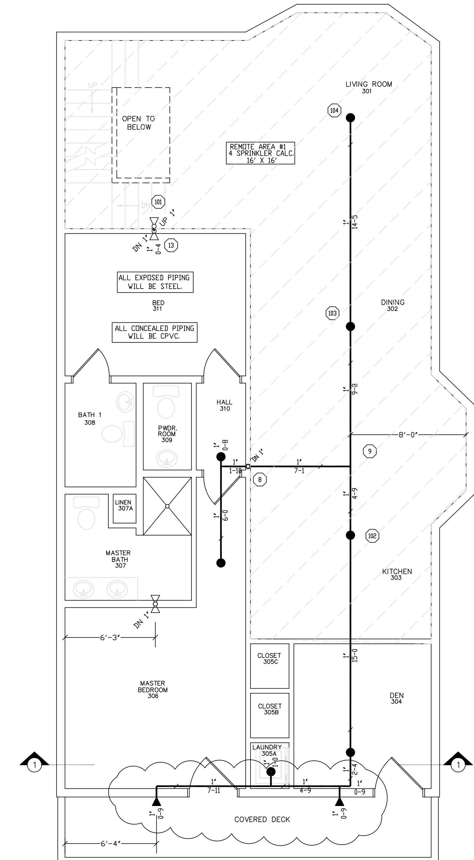
THIRD FLOOR FIRE PROTECTION SCALE 1/4"=1'-0" QUANTITY 7
