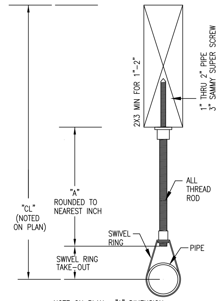
NOTE ON PLAN: "A" DIMENSION PIPE SIZES 1" THROUGH 2" - ROD SIZE 3/8" TYPE 'P' HANGER NO SCALE
