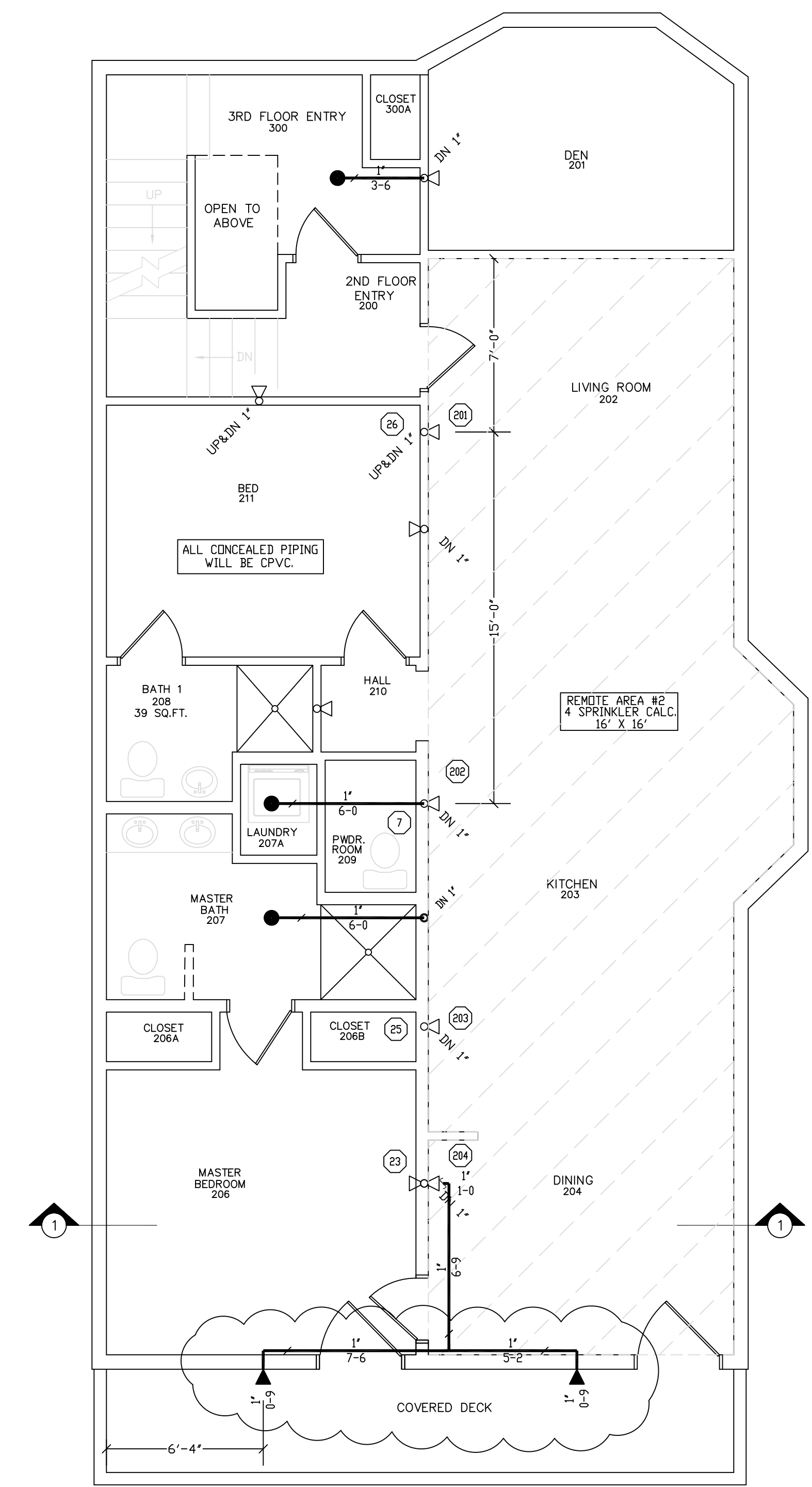
SECOND FLOOR FIRE PROTECTION SCALE 1/4"=1'-0" QUANTITY 3
