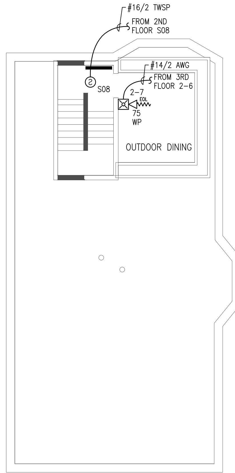
ROOF FIRE ALARM PLAN SCALE: 1/8"=1'-0"
