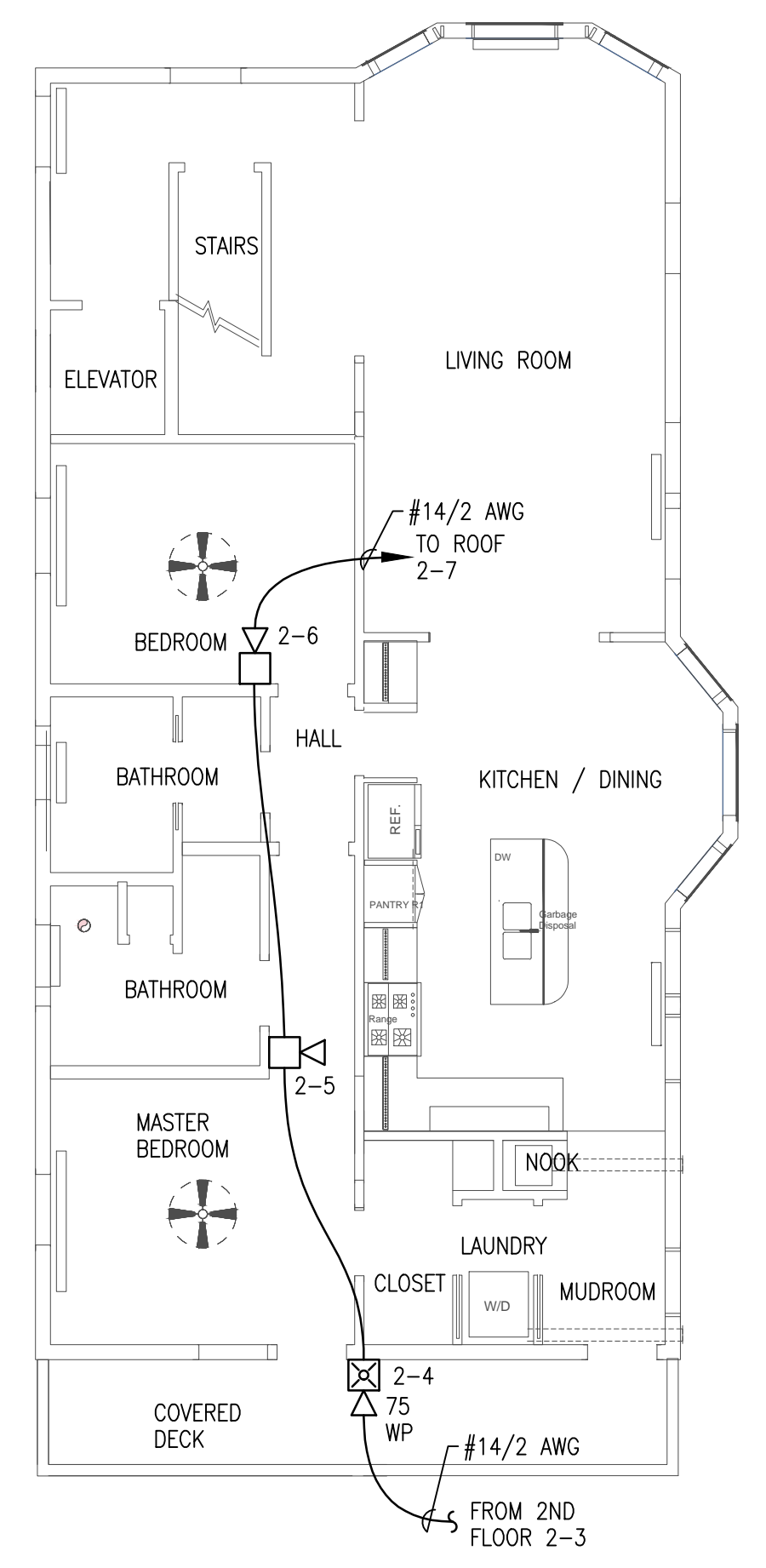
3RD FLOOR FIRE ALARM PLAN SCALE: 1/8"=1'-0" 0 4' 8' 16'
