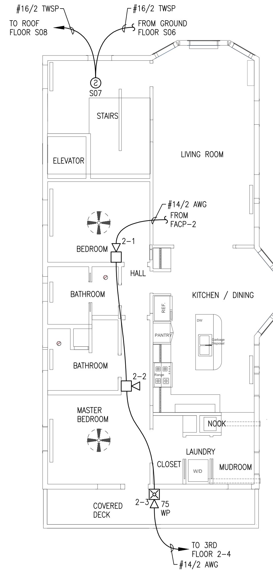
2ND FLOOR FIRE ALARM PLAN SCALE: 1/8"=1'-0"
